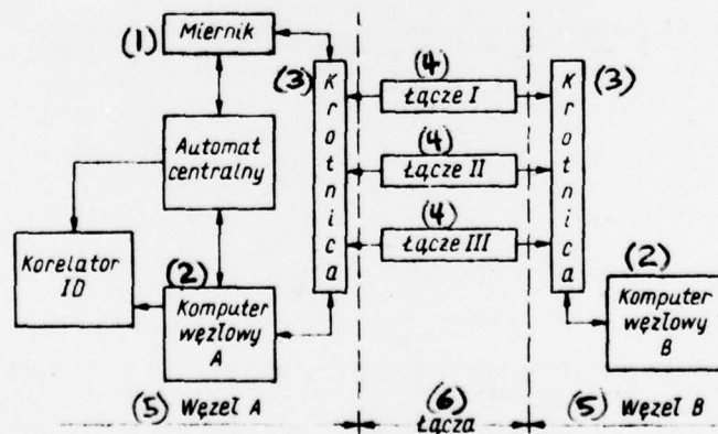
Block diagram of UKW equipment for automatic measurement and selection of basic links in activity between junctions 1 - measuring instrument; 2 - junction computer; 3 - terminal; 4 - link; 5 - junction; 6 - links
