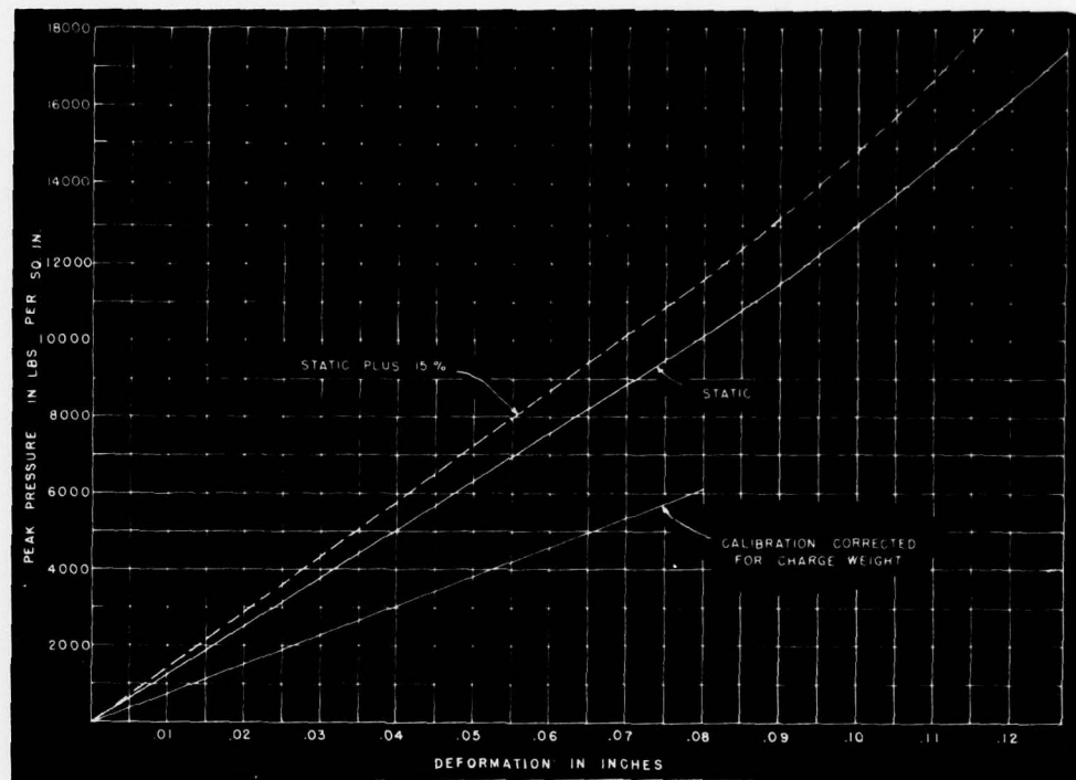
Figure 7. Calibration curves for 3/8-inch copper balls.
