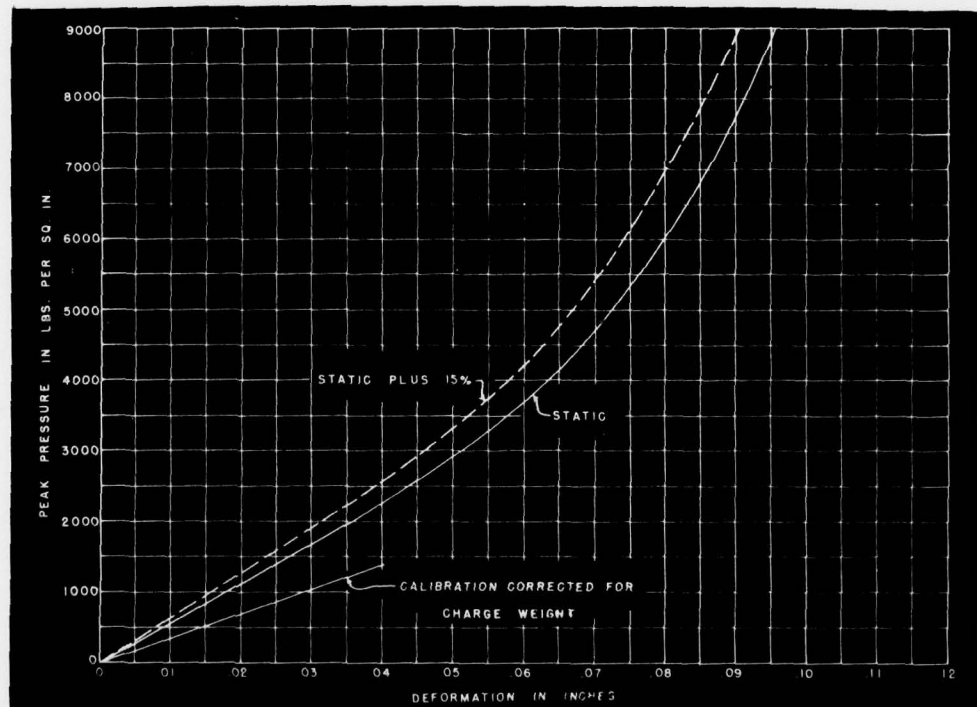
Figure 8. Calibration curves for 5/32-inch copper balls.
