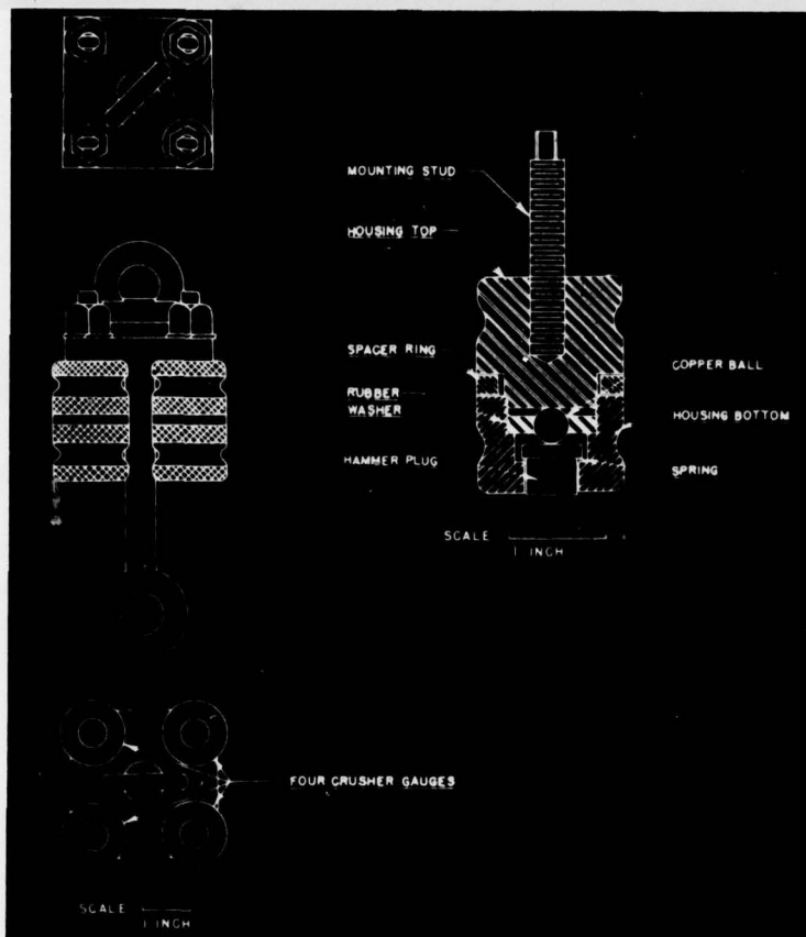
Figure 3. Ball crusher gauge and mounting block for four gauges.
