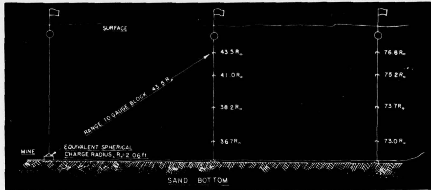
Figure 4. Experimental setup showing ranges to gauges in multiples of equivalent charge radius.
