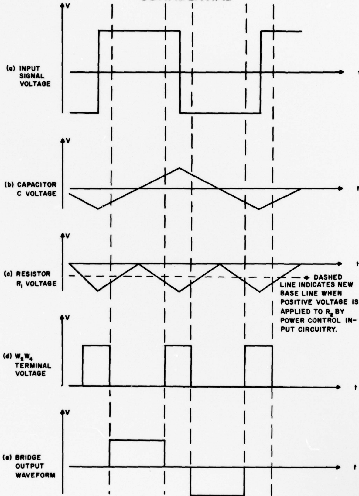
Figure 7. Amplifier Power Control Waveforms
