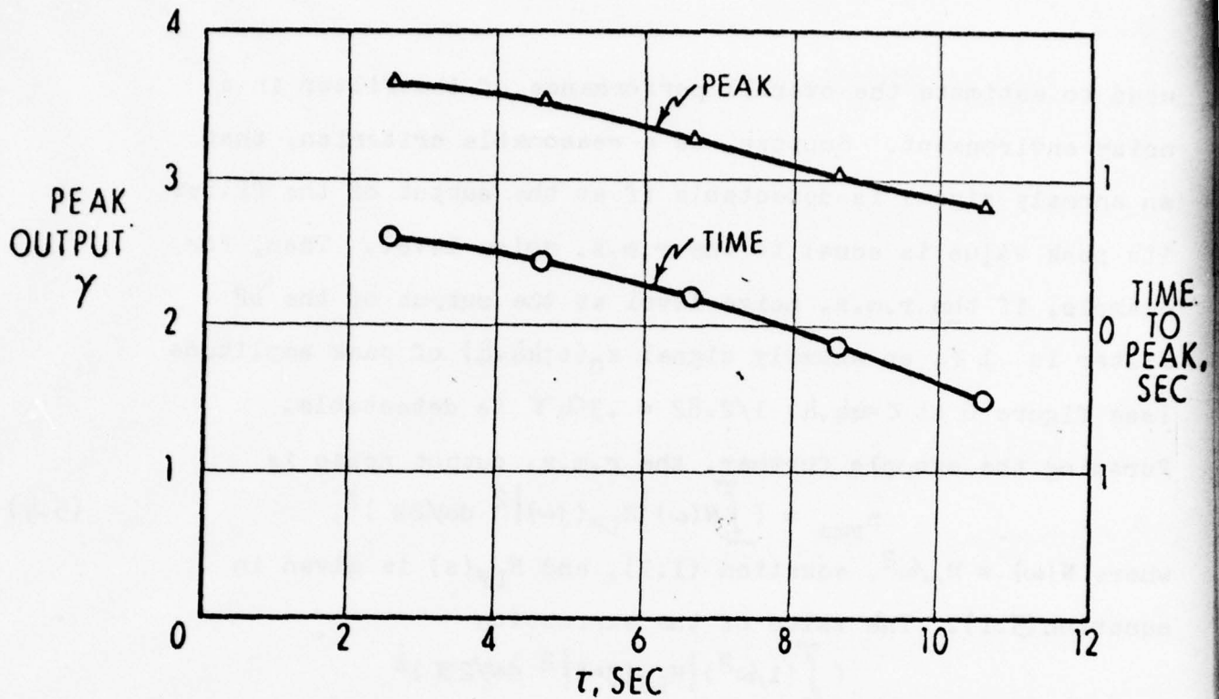
Fig. 7 HF Filter - Peak Output for 1V Peak Input and Time from Input Peak to Output Peak
