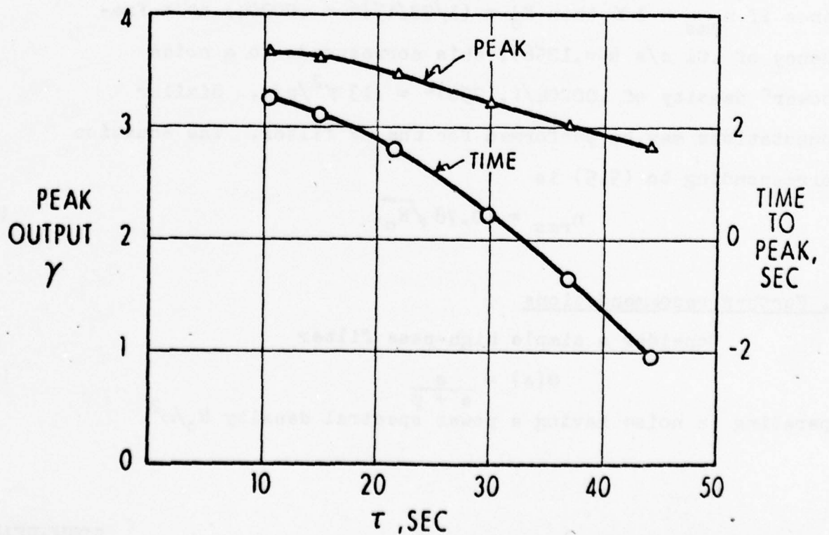
Fig. 8 LF Filter - Peak Output for 1V Peak Input and Time from Input Peak to Output Peak
