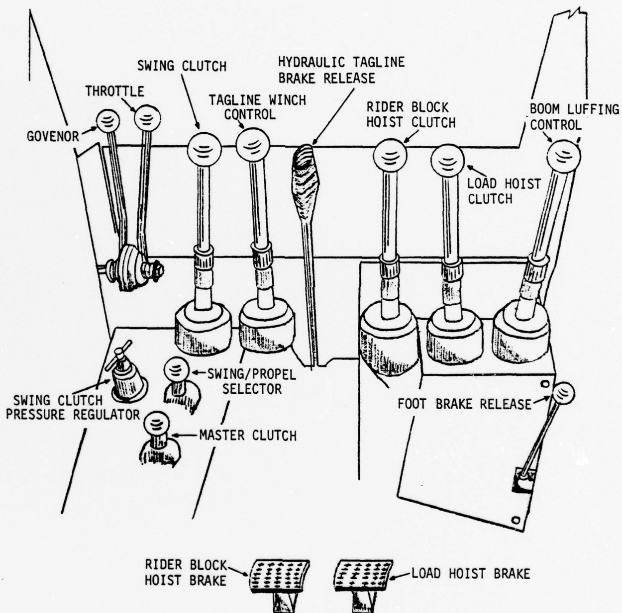
Figure 2-5. Crane Control Details
