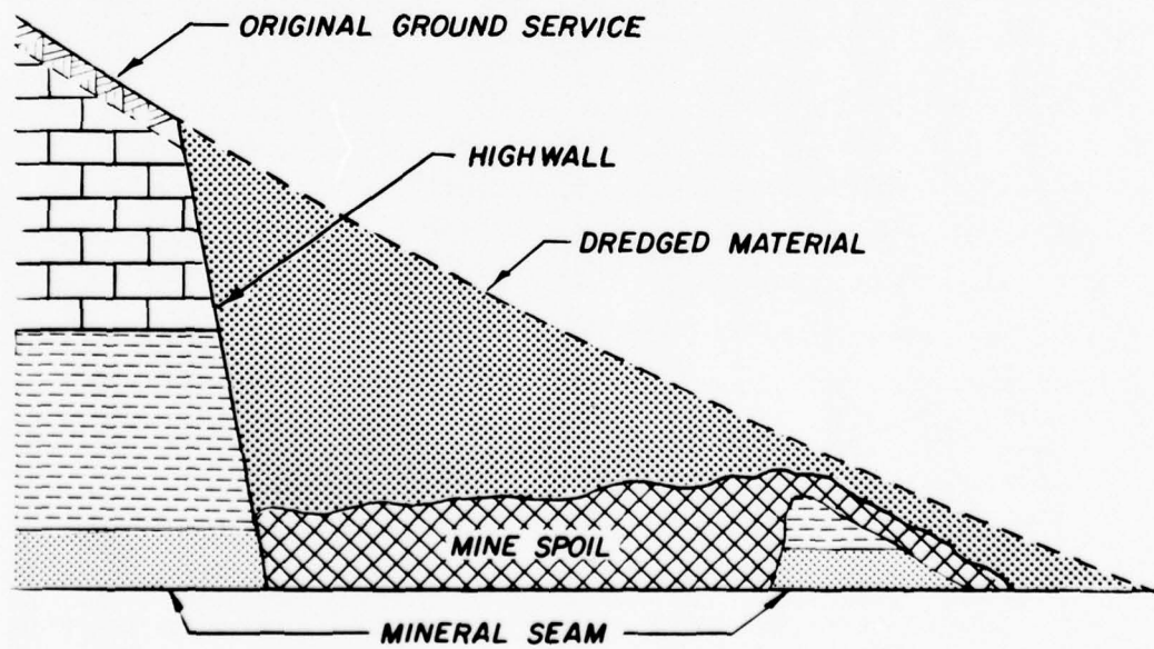
Figure 14. Cross-sectional view of contour backfill technique (from EPA 28 )
