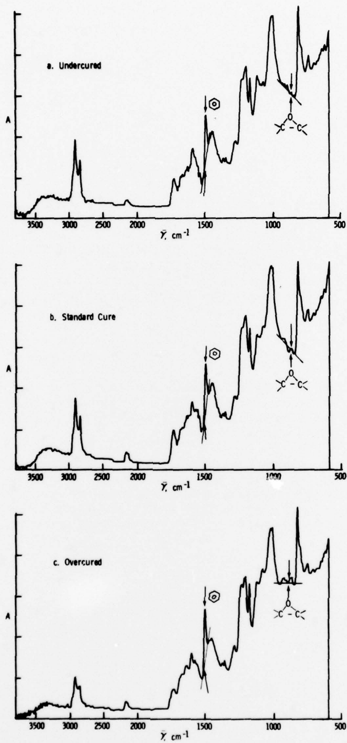
Figure 14. Internal reflectance spectrum of SP 250.
