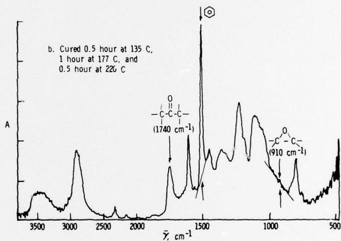
Figure 6. Infrared spectra of RAC 7250 thin film.
