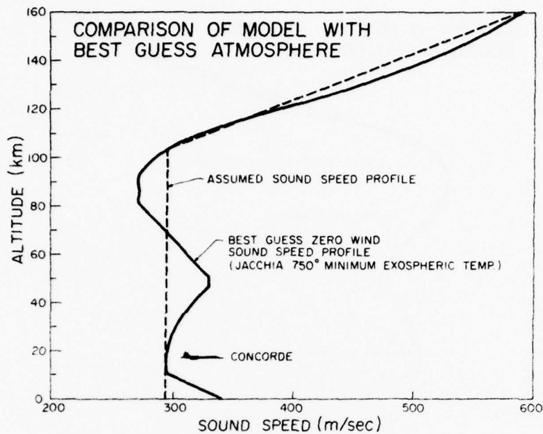
Fig. 4.2 - Comparison of sound speed for best guess atmosphere with the assumed sound speed profile
