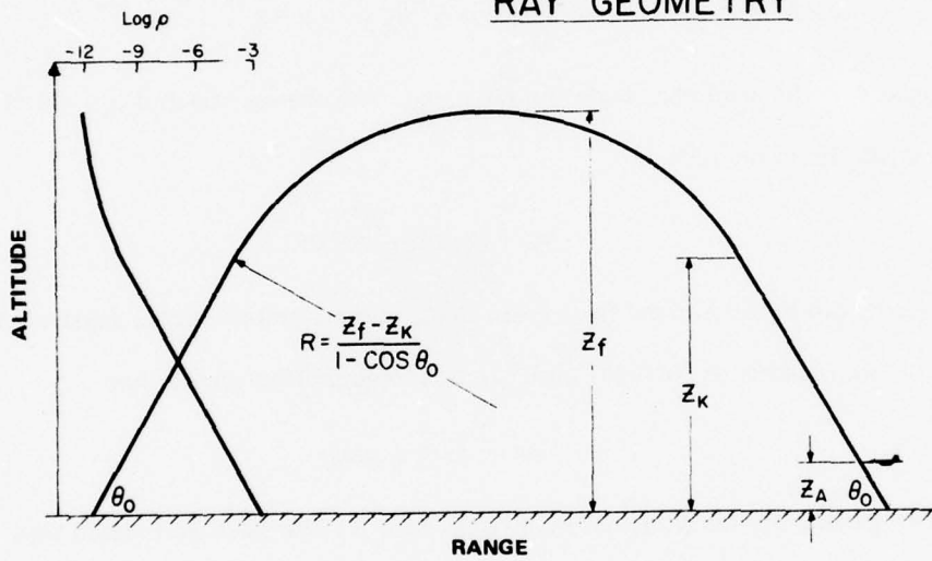
Fig. 3.2 — Ray path along ground track for model atmosphere. Note that a disproportionate amount of the path is in a region of low density causing most of the "aging" to occur at high altitudes.
