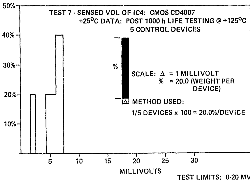
Figure 18 - Test 7, Post 1000 Hr at 125°C Data on Control Devices (25°C)
