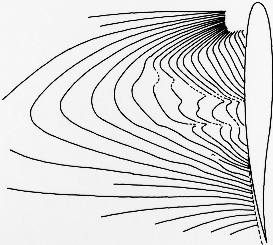
FIG. 15 INTERFEROGRAM - SUPERCRITICAL AEROFOIL BGK--1
