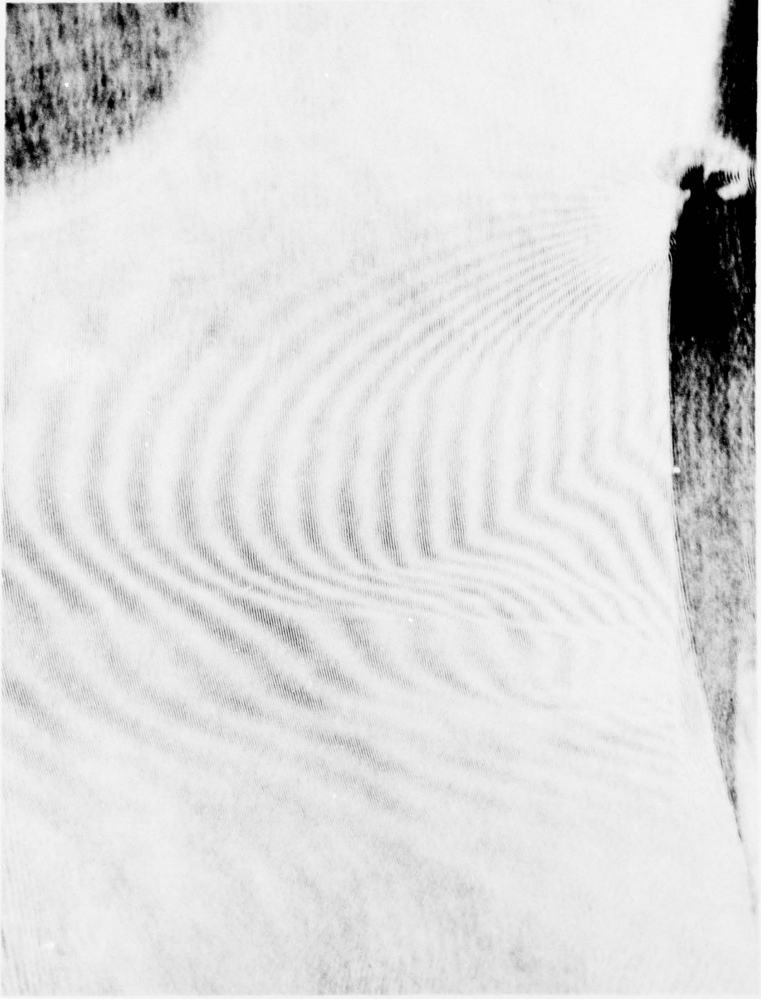
FIG. 13 COMPOSITE INTERFEROGRAM OF UPPER SURFACE FLOW ON SUPERCRITICAL AEROFOIL BGK = 1 ( M \approx 0.80 , \alpha = 1.4^\circ , R \approx 1.2 \times 10^6 )
