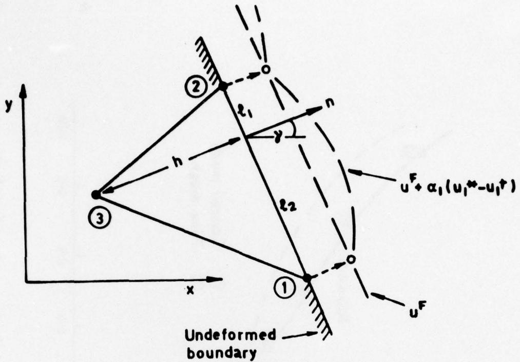
Fig 1 Element geometry and boundary displacements
