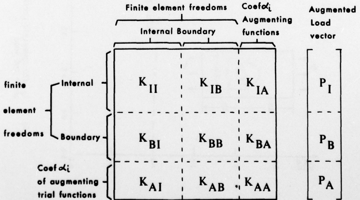
Fig 2 Partitioning of substructure stiffness matrix
