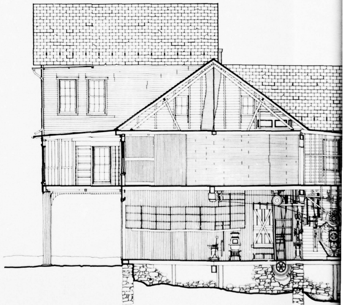
S E C T I O N T H R O U G H B L A C K S M I T
