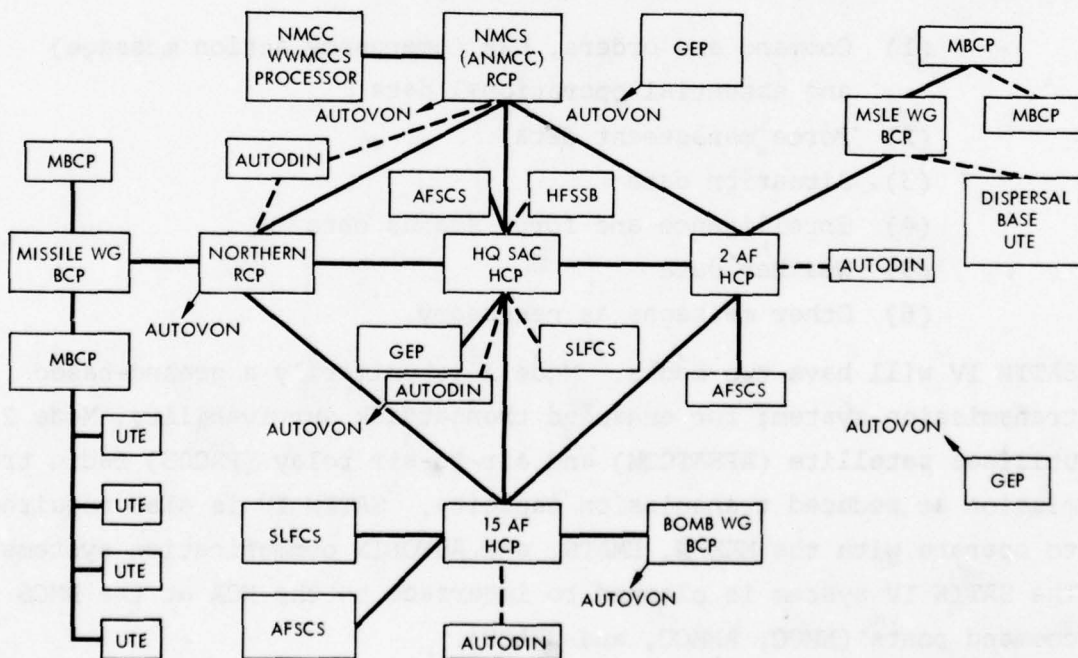
FIGURE 2. Proposed SATIN IV Network (Ref. 6)
