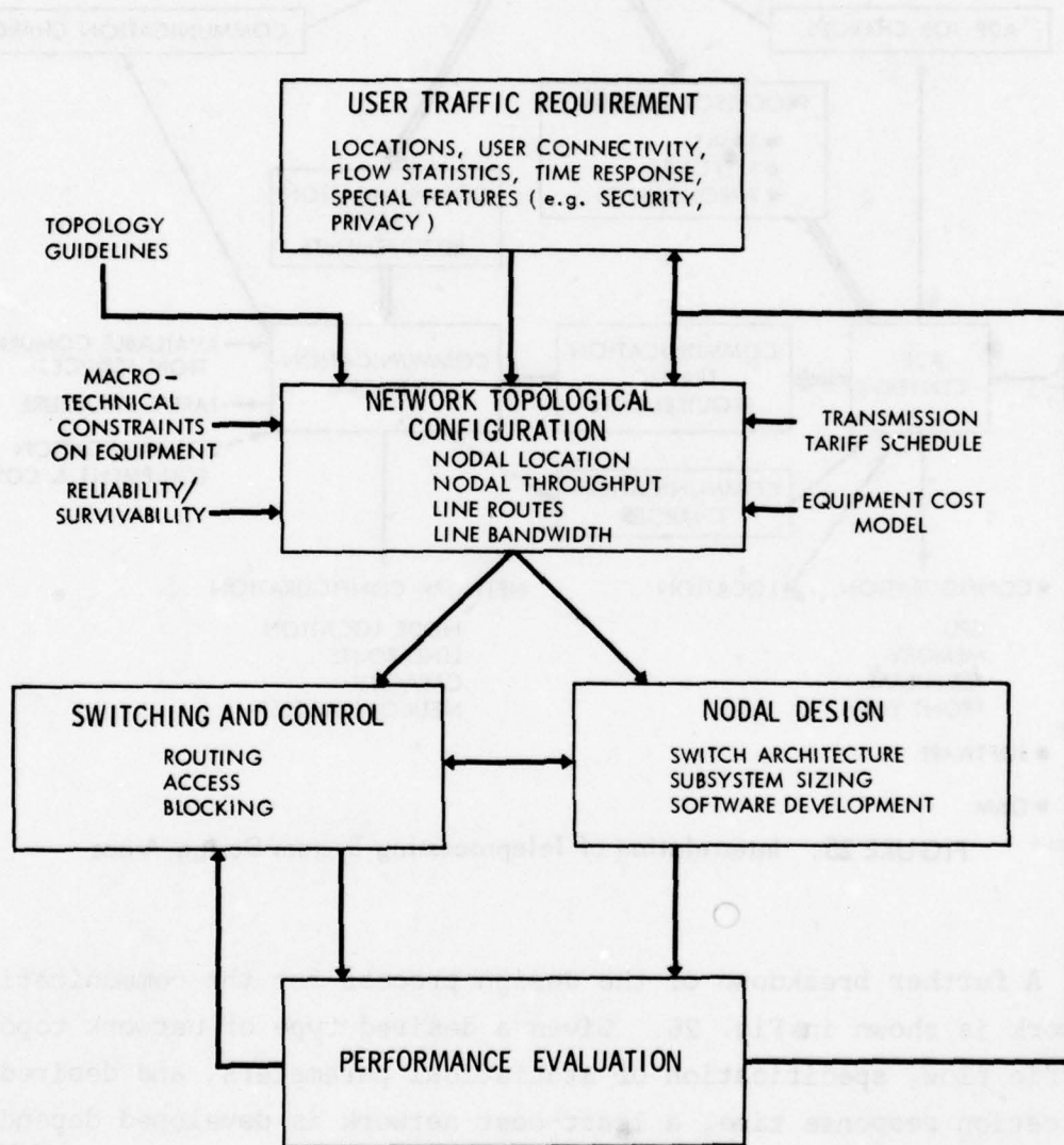
FIGURE 26. Teleprocessing Communication Network Design Process
