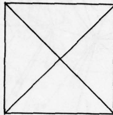
n=4, m=3
