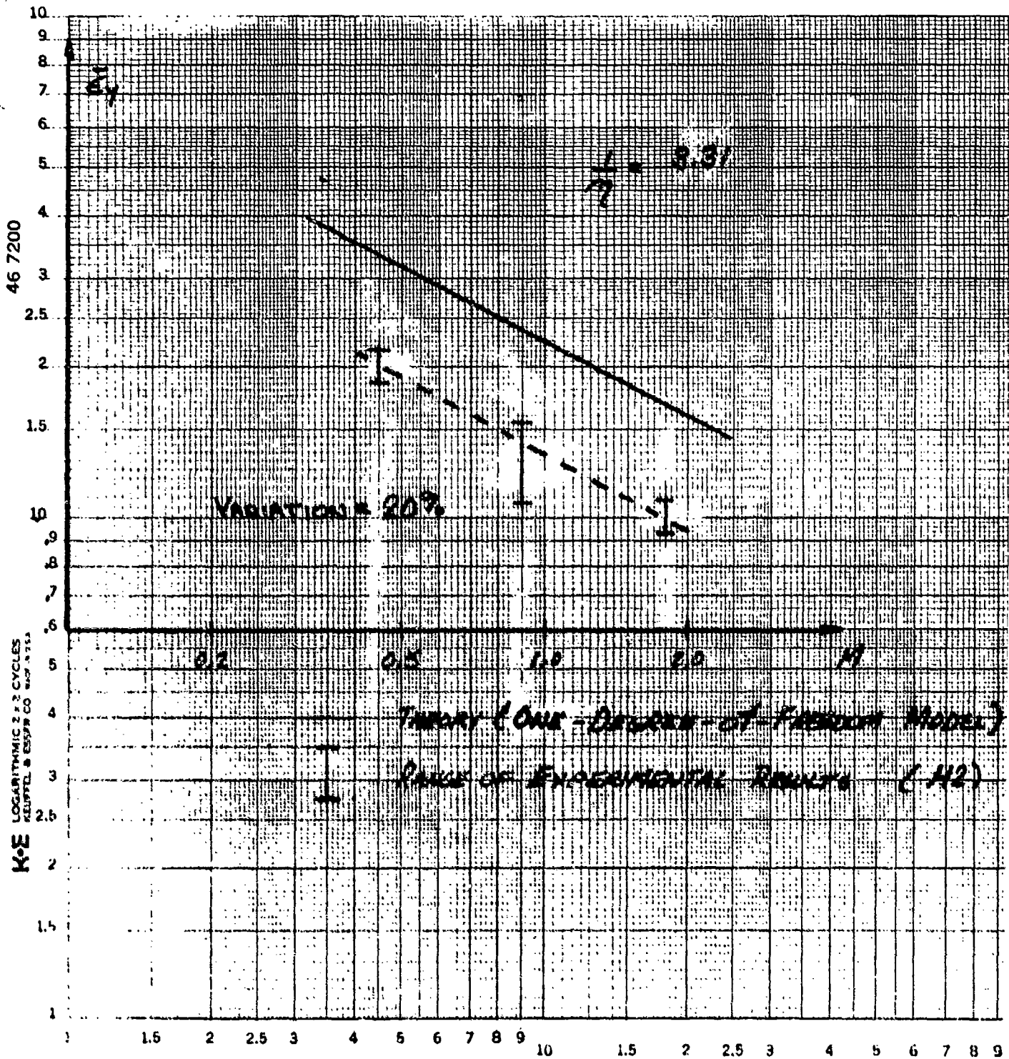
Figure E41. \bar{\epsilon}_y vs. M : Simply Supported Orthotropic Plate
