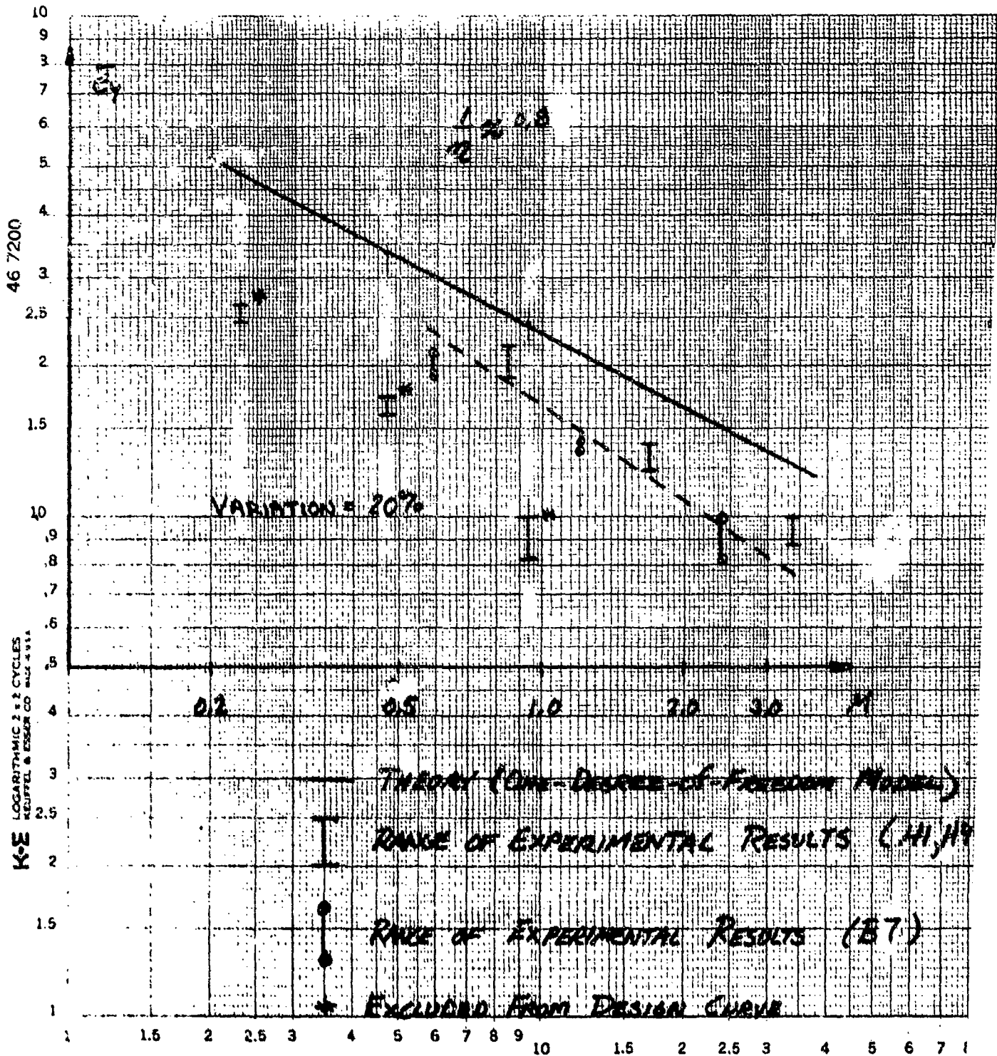
Figure E39. \bar{\epsilon}_y vs. M : Simply Supported Orthotropic Plate
