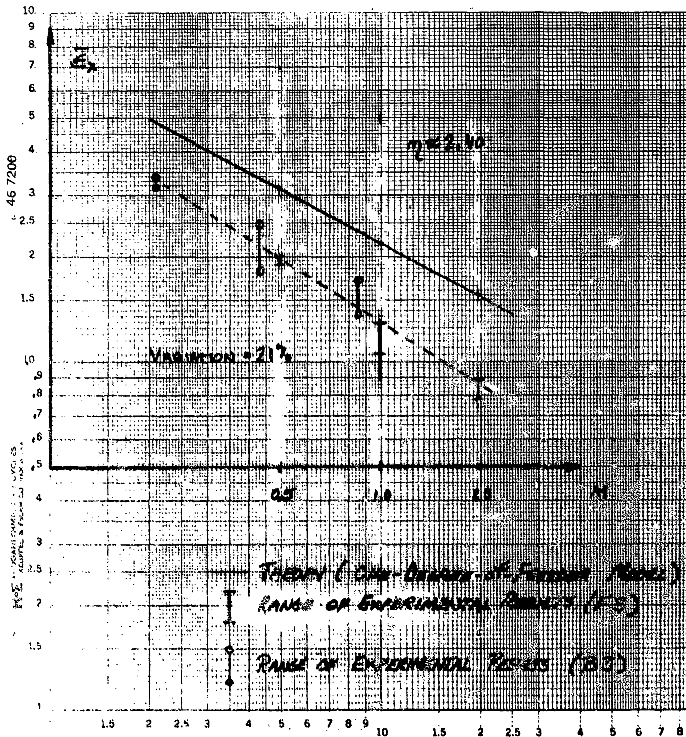
Figure B32. \bar{E}_x vs. H : Simply Supported Orthotropic Plate
