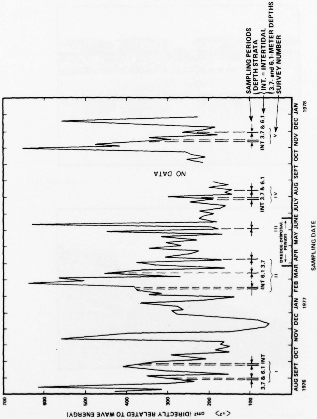
Figure 7. Wave energies for Imperial Beach expressed in terms of \langle n^2 \rangle cm 2 .
