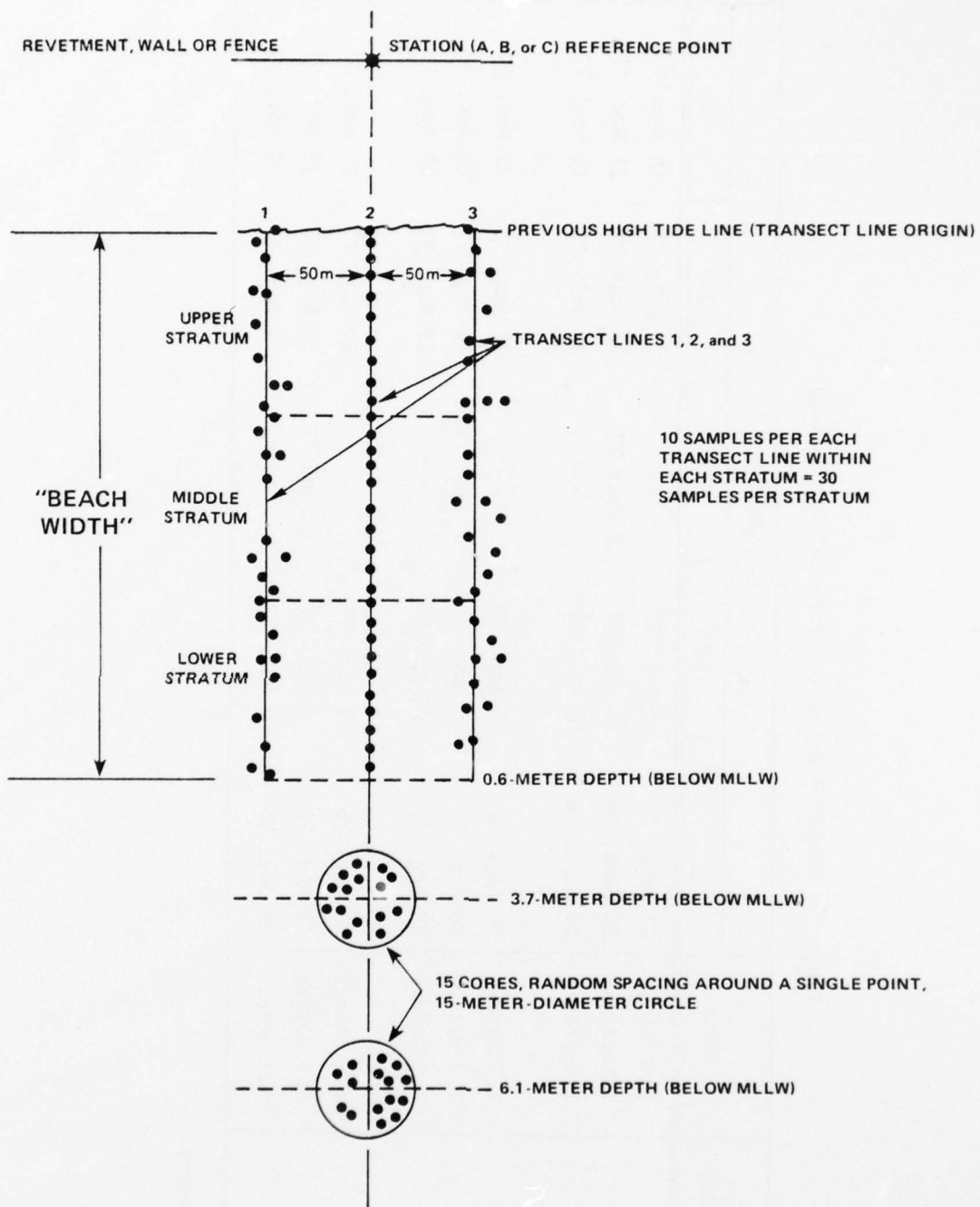
Figure 2. Single station sampling scheme (not to scale).
