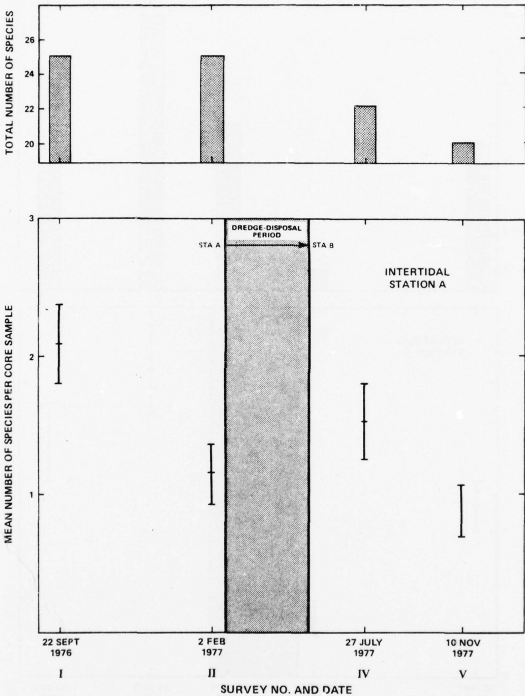
Figure 23. Mean number of species per core sample and total species sampled per survey for intertidal station A. Bars = \bar{X} \pm t_{.95} \frac{S}{\sqrt{X}} .
