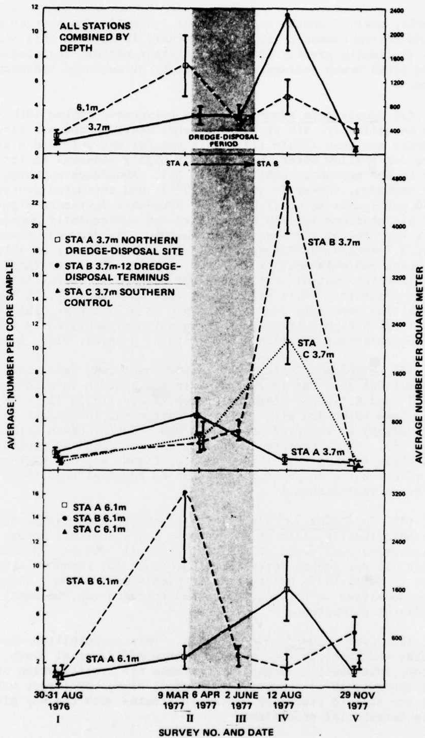
Figure 37. Mean number per core sample and estimated abundances per square meter for Apoprionospio pygmaea (polychaete) at 3.7- and 6.1-meter stations.
