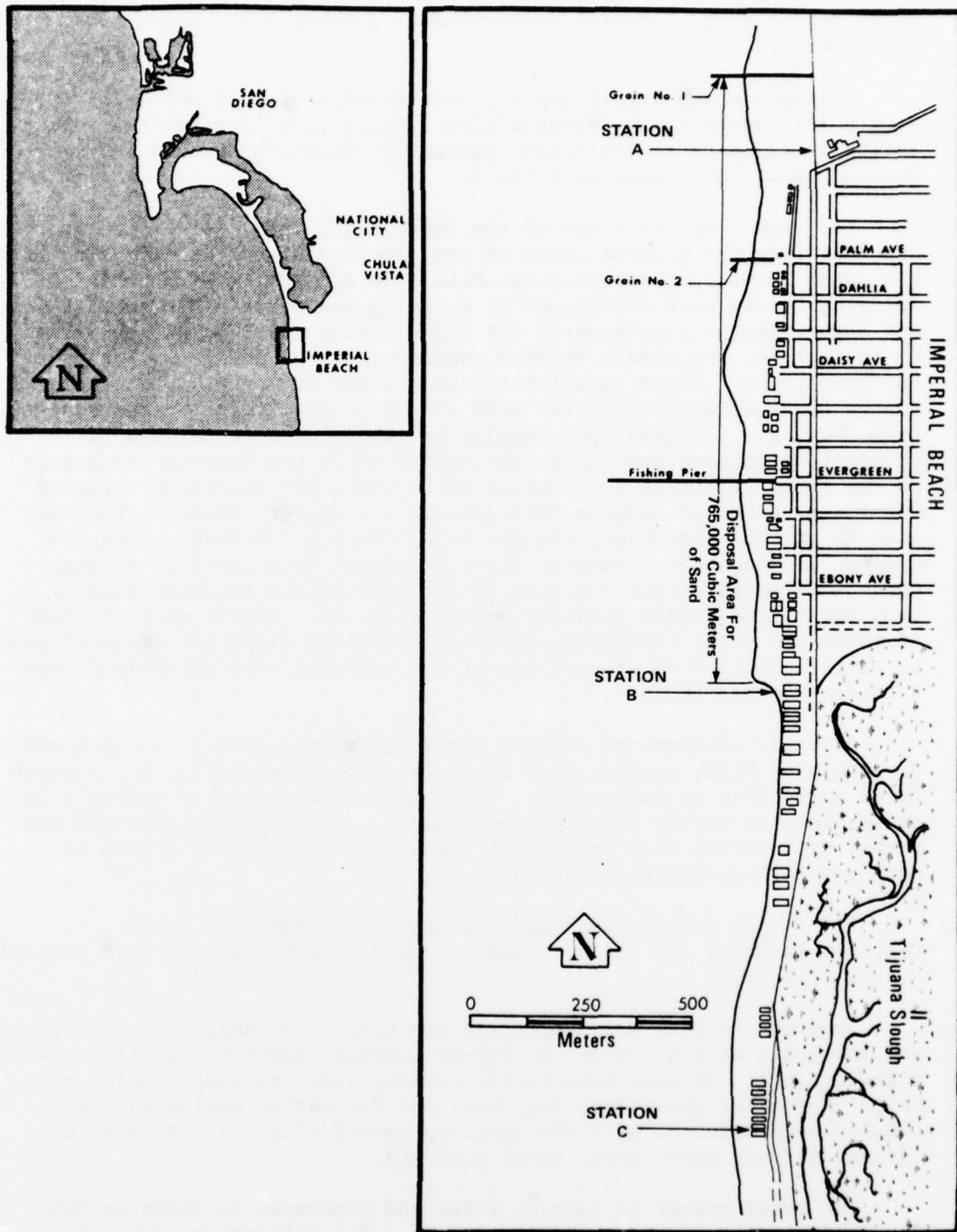
Figure 1. Location of sampling stations at Imperial Beach, California.
