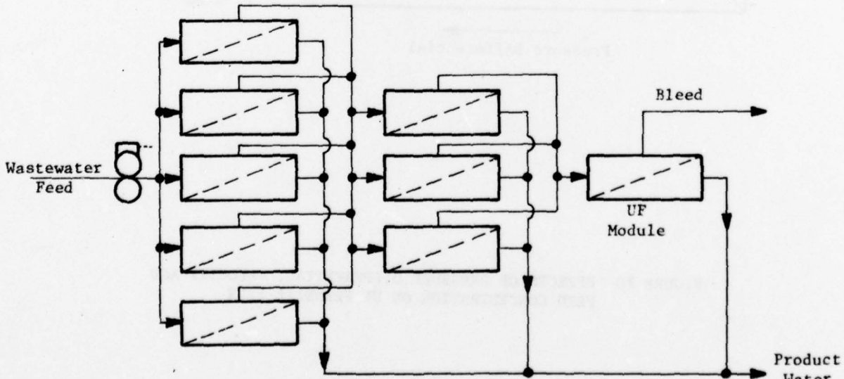
(c) Continuous Once-Through
