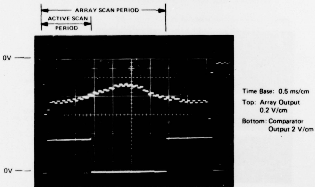
Fig. 10. Array response to 23-mil line for 1/8-inch fiber optics.
