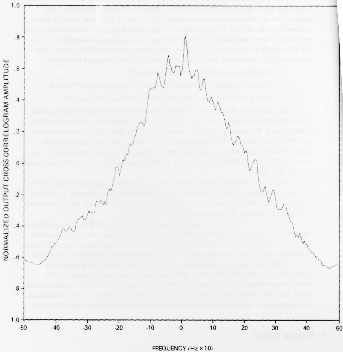
(C) Figure 6(b). Simulated Output Correlogram for the Frequency-Domain Implementation of STARLITE: \phi = 45^\circ , R = 5 Kyd, \beta = 90^\circ , S-N-R = 0 dB.
