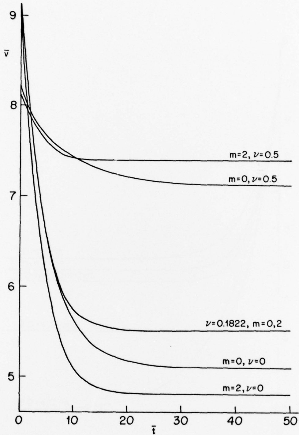
Figure 10 - Radial Velocity \bar{v} vs. \bar{t} at \bar{r} = 1.0 - Case I-b
