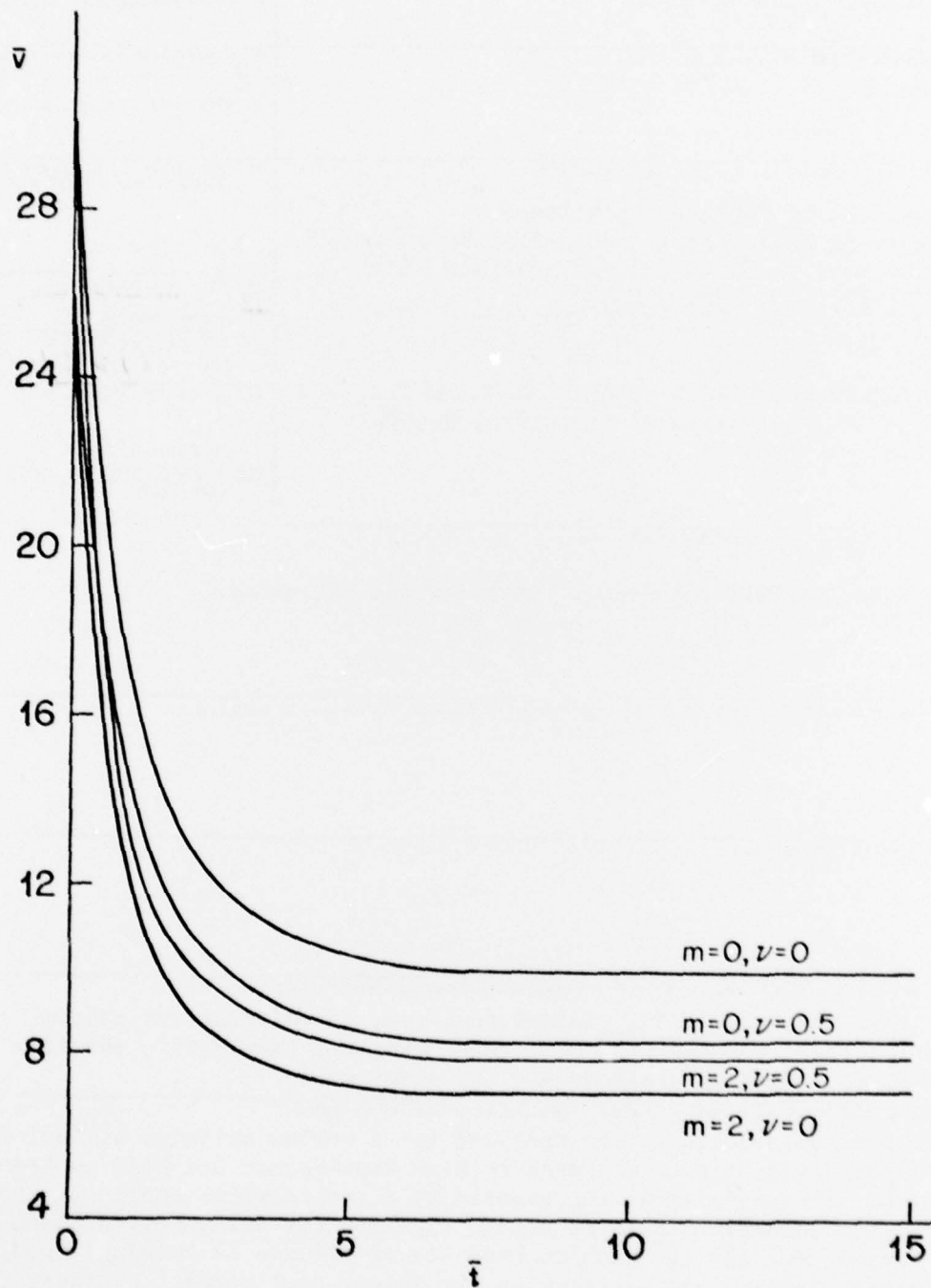
Figure 11 - Radial Velocity \bar{v} vs. \bar{t} at \bar{r} = 1.0 - Case II
