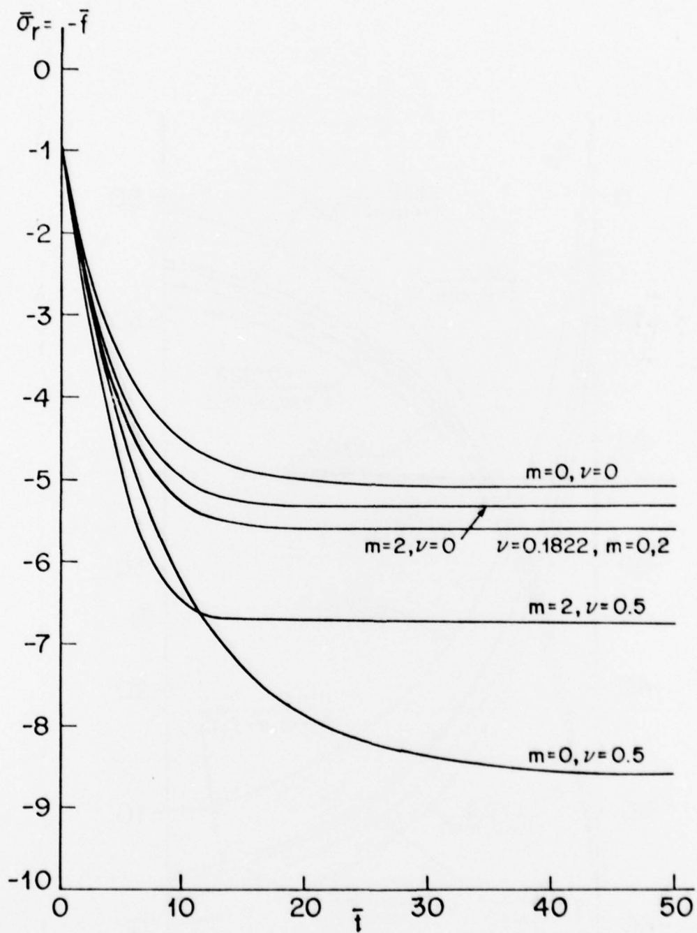
Figure 8 - Radial Stress \bar{\sigma}_r vs. \bar{f} at \bar{r}=1.0 - Case I-b
