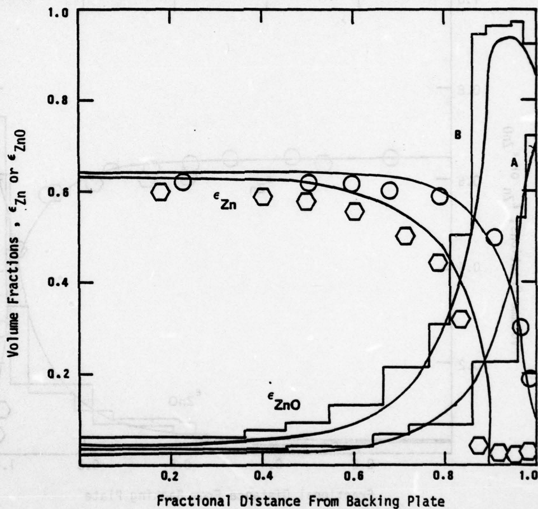
Figure 18. Profiles of Zn (Circles and Hexagons) and ZnO (Histograms) for the Low Porosity Electrode Discharged at 20 mA/cm 2 . \circ and Histogram A, Measured Profiles After 10% Depth; \hexagon and Histogram B, Measured Profiles After 23% Depth; Smooth Curves, Predicted Profiles After 10% and 23% Depths of Discharge.
