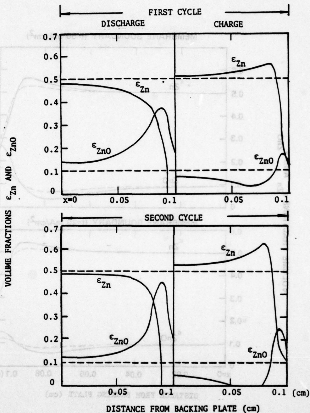
Figure 12. Distribution of Zn and ZnO Plotted As Volume Fractions ( \text{cm}^3/\text{cm}^3 ) During Two Cycles for Solution Boundary ( I=50 \text{ mA}/\text{cm}^2 , L=0.1 \text{ cm} , \epsilon_{\text{Zn}}^0 = 0.5 , \epsilon_{\text{ZnO}}^0 = 0.1 )
