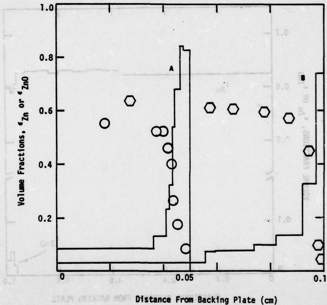
Figure 22. Profiles of Zn (Circles and Hexagons) and ZnO (Histograms) Measured for the Low Porosity Electrode Discharged At 50 \text{ mA/cm}^2 . \bigcirc and Histogram A for 20% Depth of Discharge for the Electrode Having Thickness of 0.05 cm; \hexagon and Histogram B for 8% Depth of Discharge for the Electrode Having Thickness of 0.1 cm.
