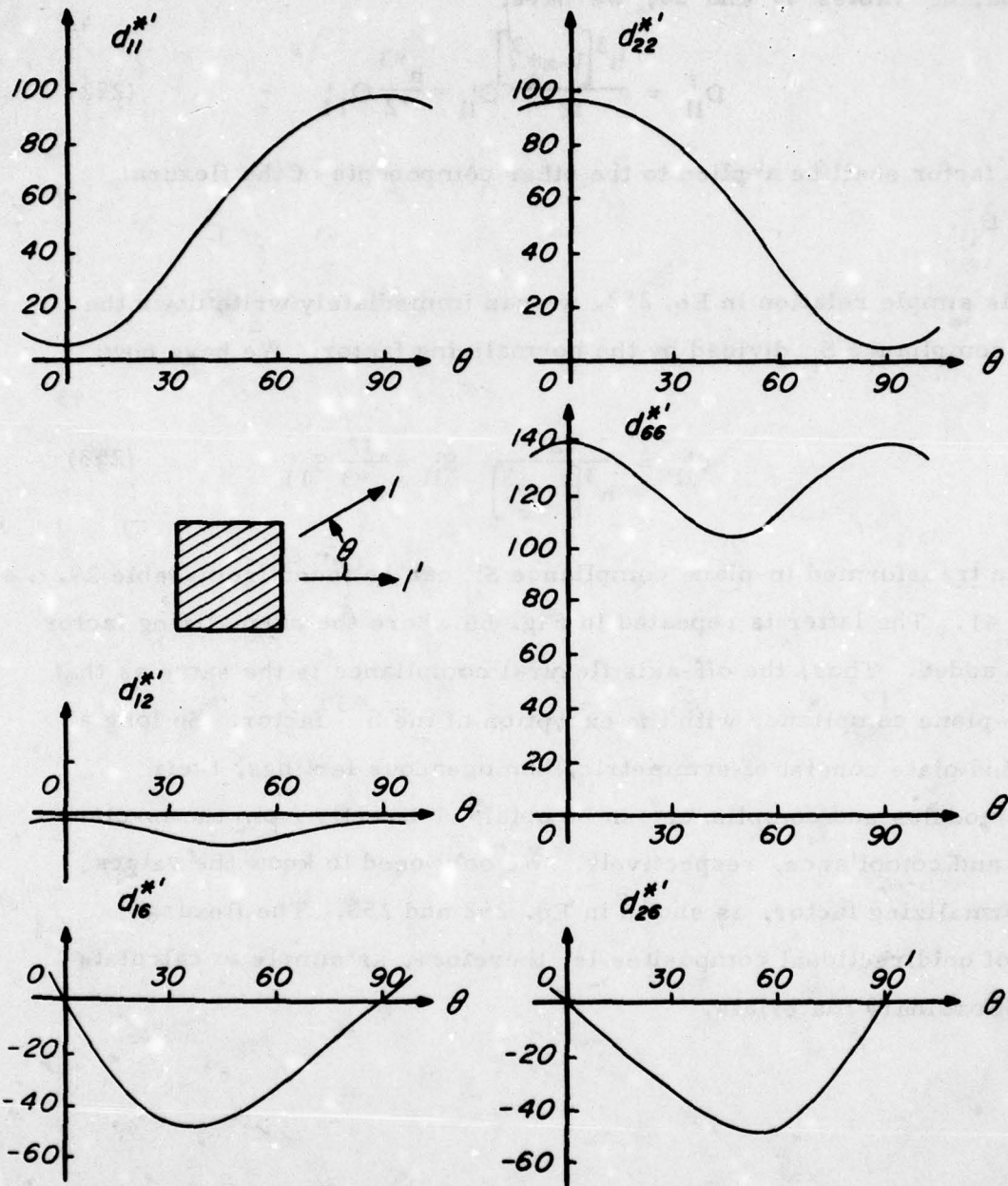
Fig. 66. Transformed flexural compliance of unidirectional T300/5208. This is the same as Fig. 41 for the off-axis compliance except the normalizing factor h^{*3} has been added.
