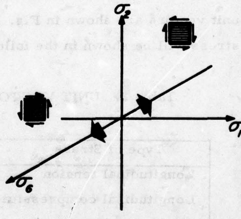
Fig. 5. Positive and negative longitudinal shears. The respective unit vectors are (0, 0, \pm 1) .
