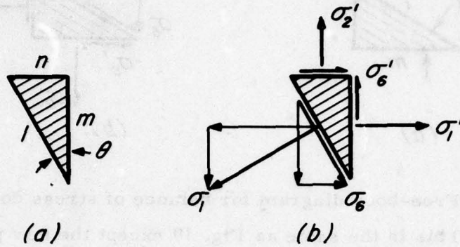
Fig. 19. Free-body diagram for the balance of stress components. The components of on-axis, 1-2 coordinates can be expressed in terms of those of the off-axis, 1'-2' coordinates. All stress components shown are positive.
