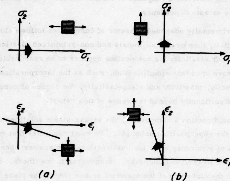
Fig. 9. Unit strain vectors resulting from uniaxial stresses
