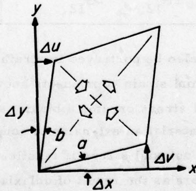
Fig. 8. The strain-displacement relation for shear strain. The arrows show the direction of stretching and compressing the diagonals.
