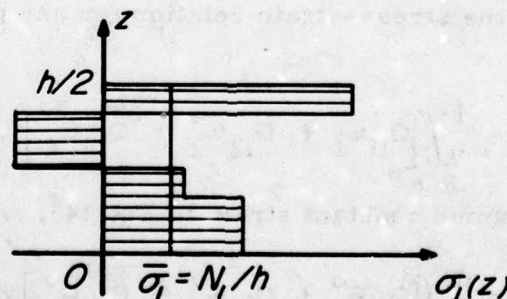
Fig. 48. Definition of average stress. Comparison between the corresponding components of the actual ply stress and the average laminate stress is shown.
