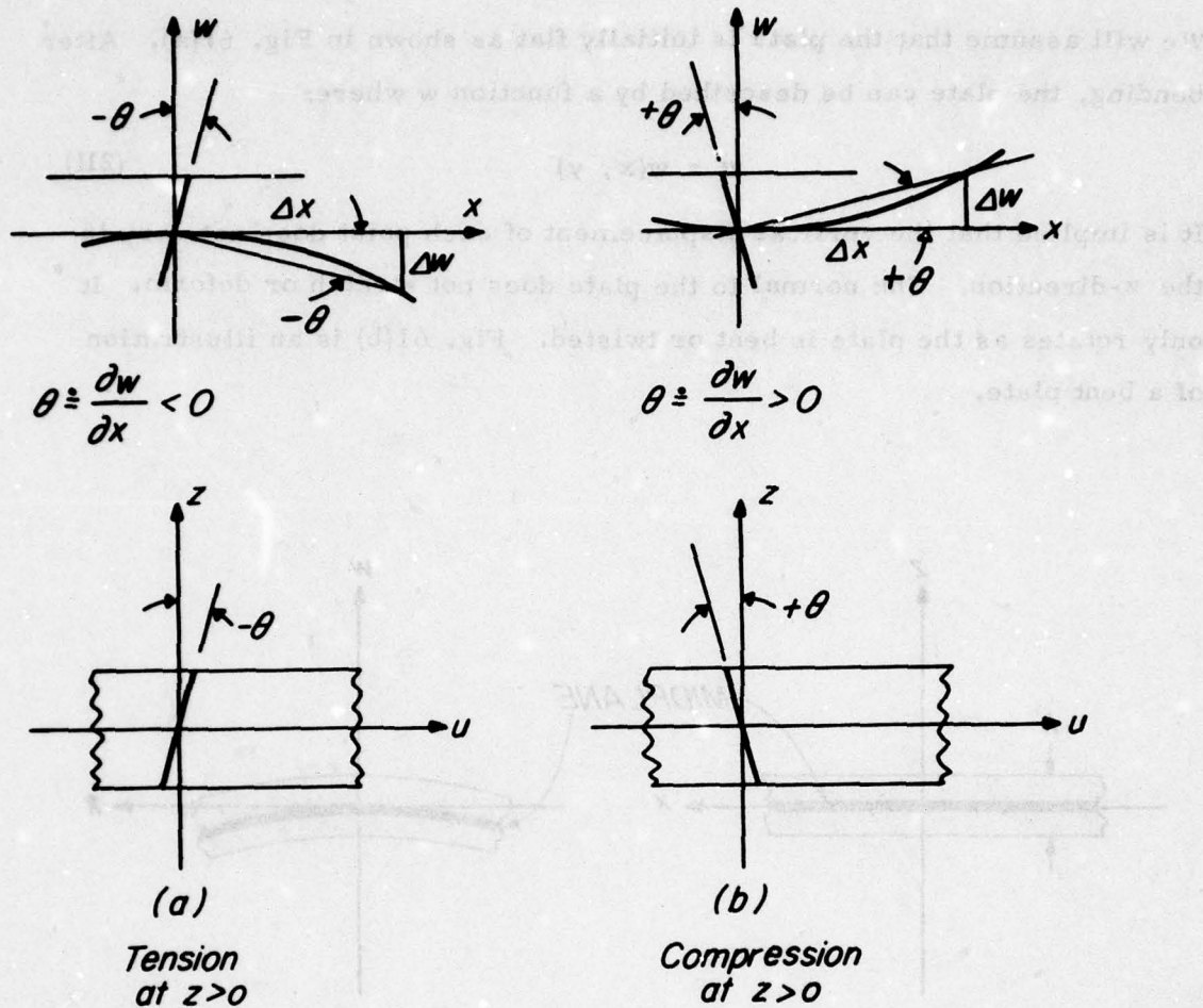
Fig. 62. Sign convention of midplane displacements. For a concave downward deformation in (a), the derivative of w is negative, and a negative sign must be added to the displacement-derivative relation in Eq. 212. When the curvature is reversed in (b), the derivative of w is now positive.
