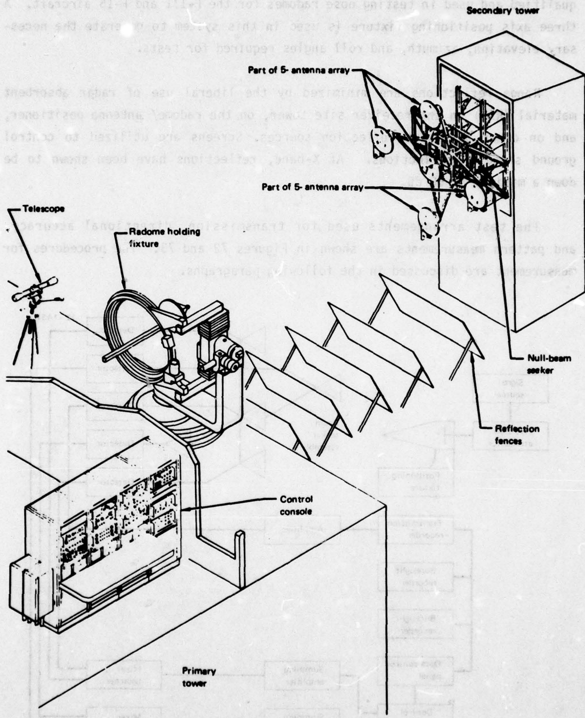
Figure 71 Brunswick radome test range
