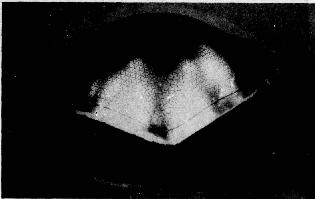
Figure 65 Mandrel for electroforming the radome nose cap
