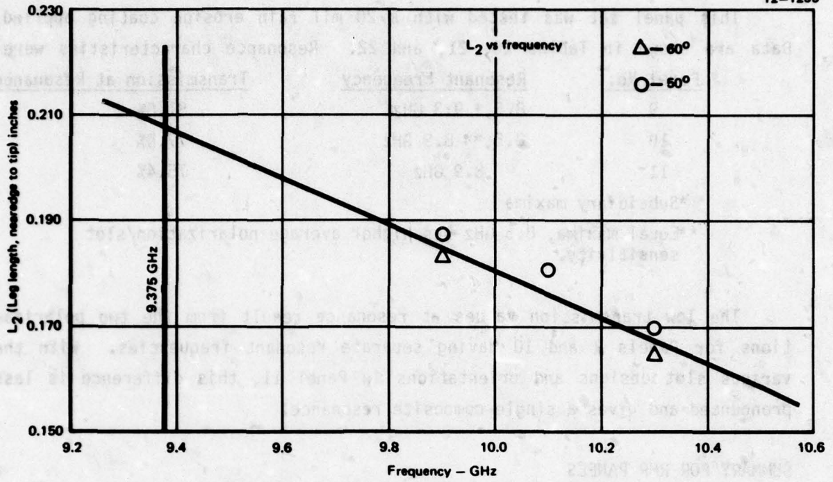
Figure 61 (L 2 leg length, near edge to tip) versus frequency
