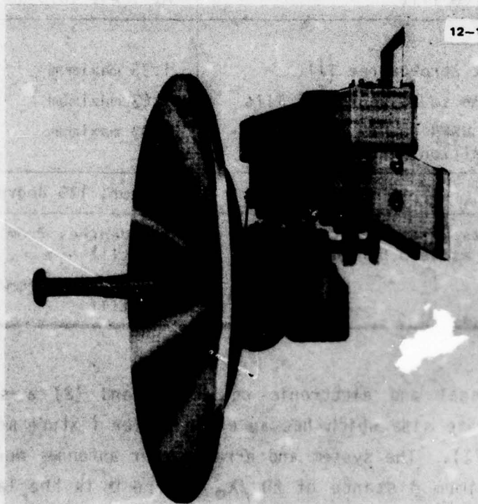
Figure 70 ANT-1G (X-band) sector scanning antenna
