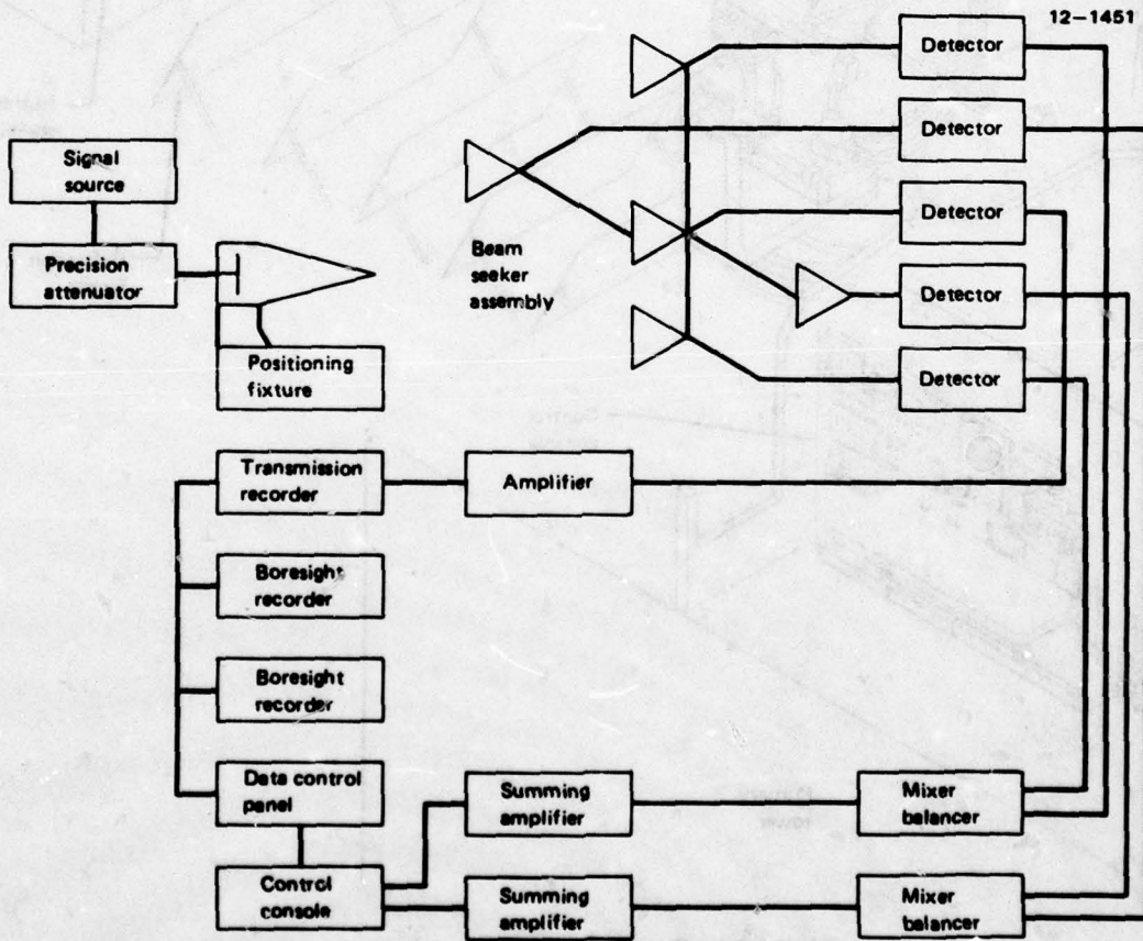
Figure 72 Test arrangement, transmission and directional accuracy
