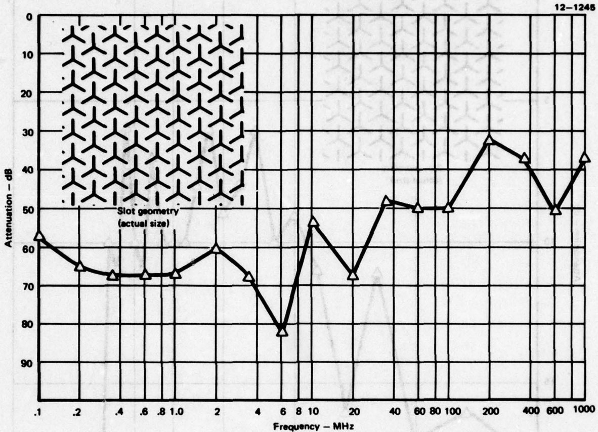
Figure 41 Attenuation of a singly coated specimen. (0.1 MHz - 1000 MHz)
