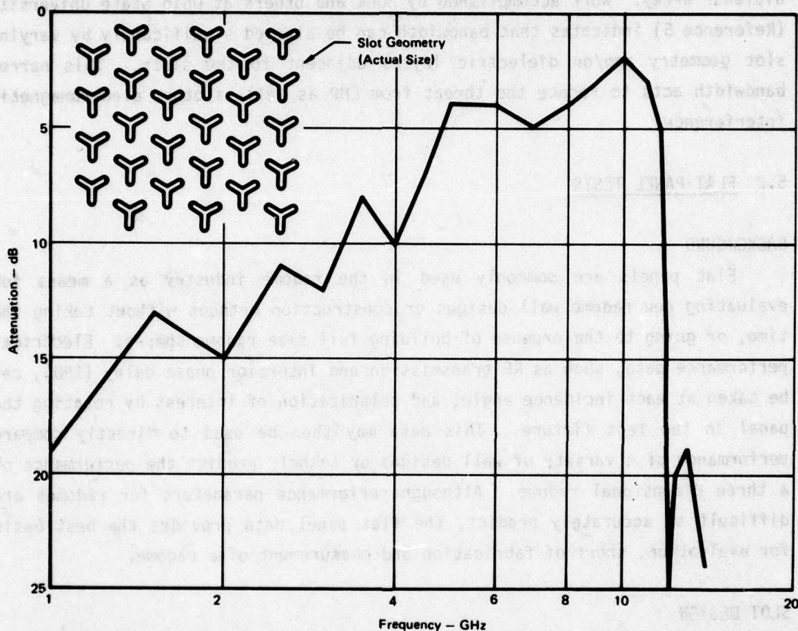
Figure 45 Attenuation of a singly coated specimen centerloaded design (1 GHz - 15 GHz)
