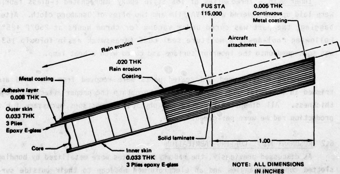
VIEW A
