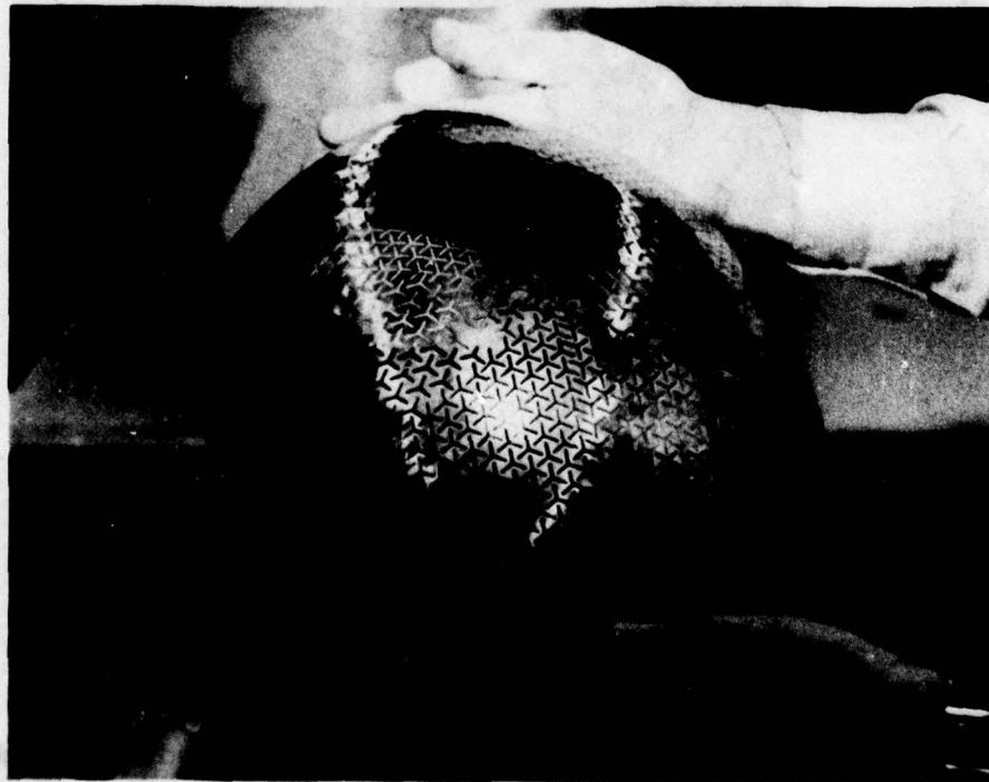
Figure 66 Electroformed copper nose cap for the demonstration radome
