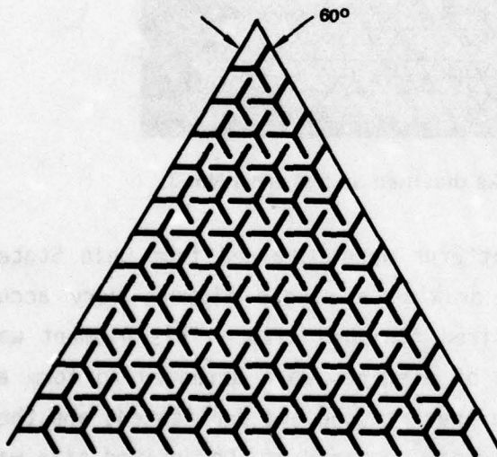
Figure 49 Slot patterns with 60° and 70° grid angles as used on the 60° and 70° triangles
