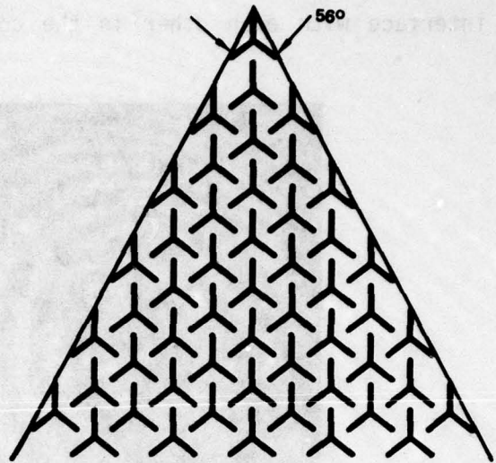
Figure 48 Slot patterns with 50° and 56° grid angles as used on the 50° and 56° triangles
