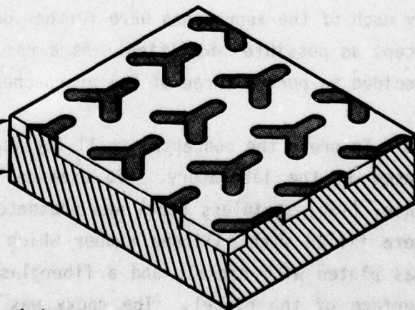
Figure 4 Raised slot approach
