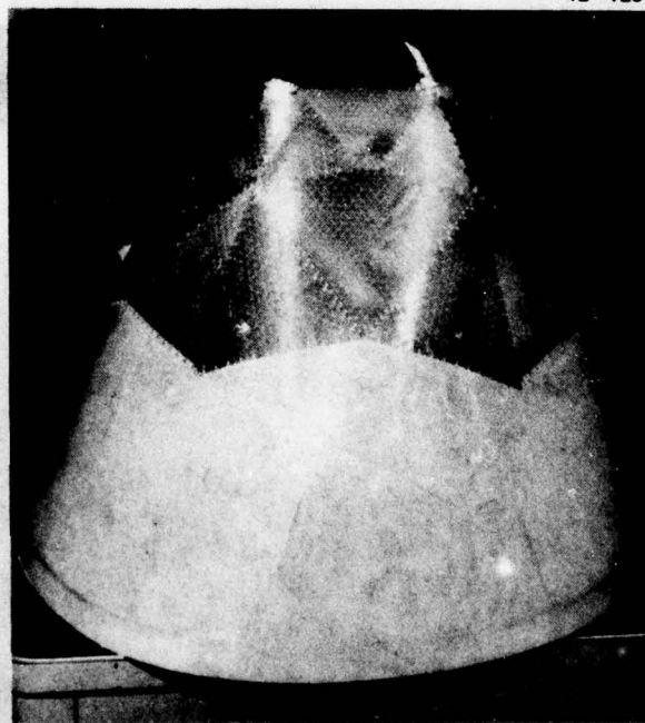
Figure 67 Demonstration radome, coated with AF 147 film adhesive and some triangles in place.
