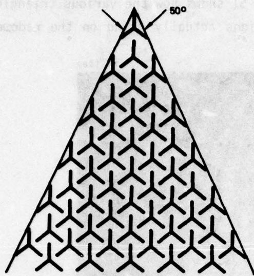
Figure 48 Slot patterns with 50° and 56° grid angles as used on the 50° and 56° triangles
