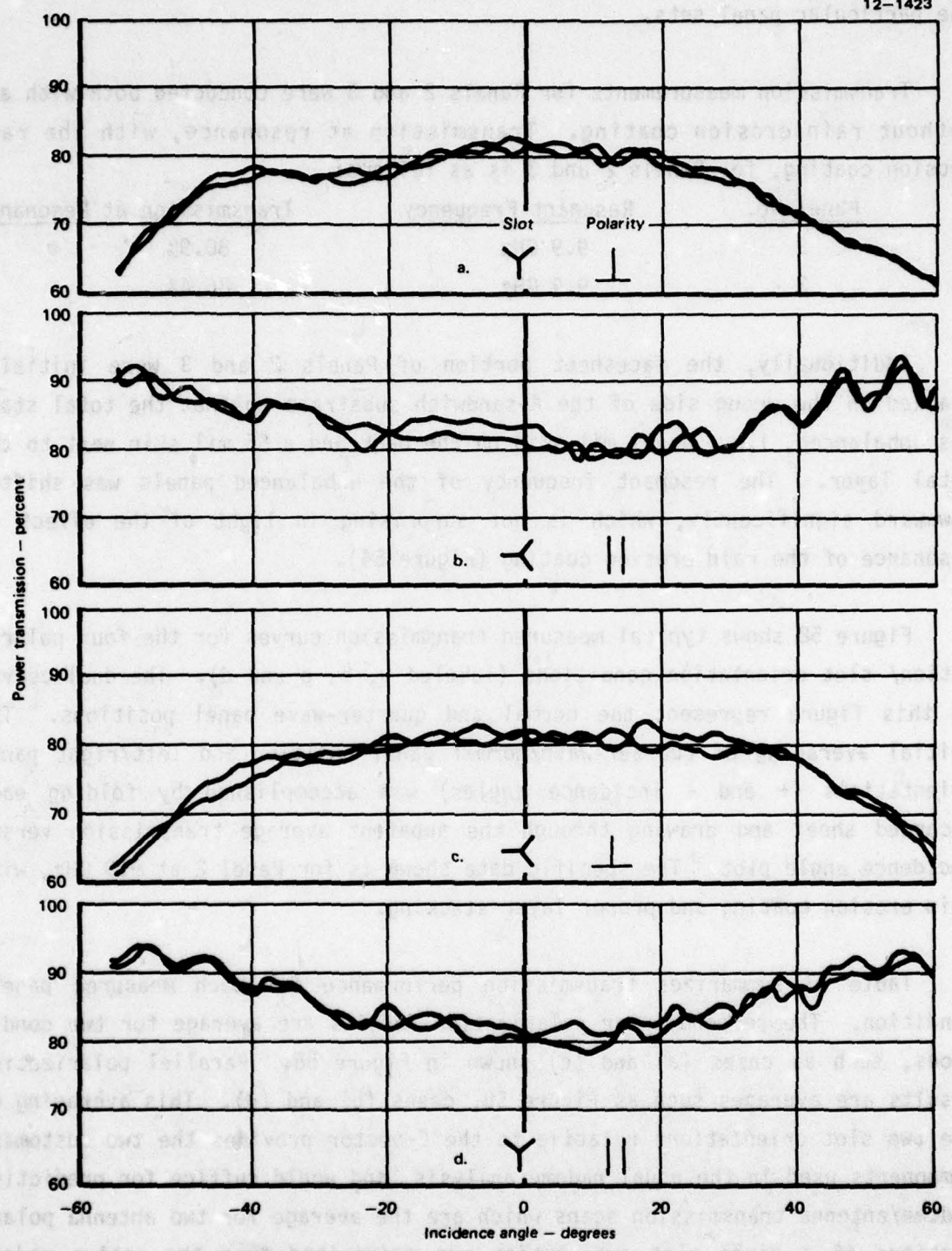
Figure 58 Measured transmission, RMR panel no. 2, 9.9 ghz, four polarization/slot orientation conditions
