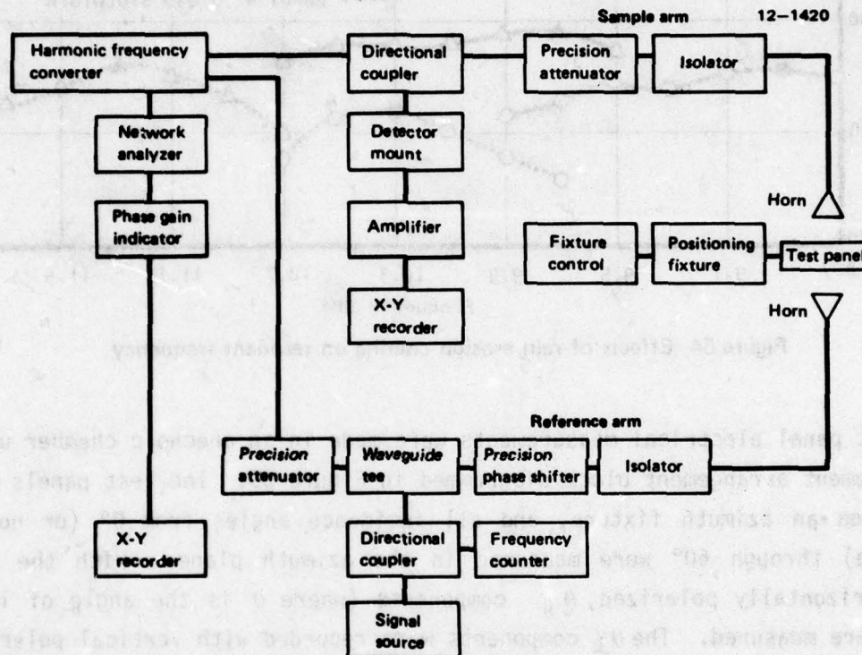
Figure 55 Test arrangement, flat panel tests
