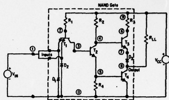
Fig. 3 Schematic diagram of a 7400 NAND gate with external connections. Node numbers used in SPICE simulations are shown.
