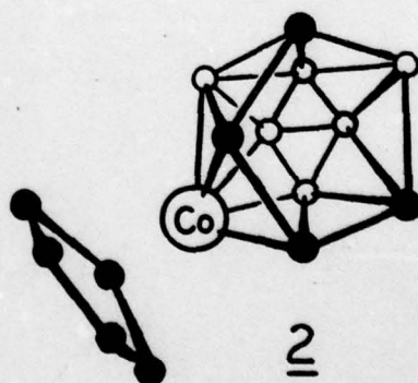
ISOMER I
