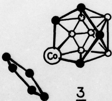
ISOMER II
