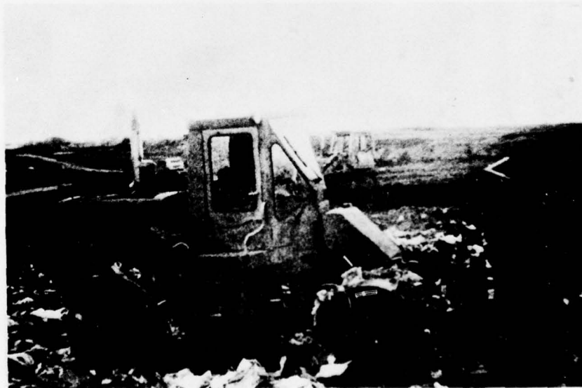
Figure 6. Steel-wheeled vehicle with widely spaced cleats.
