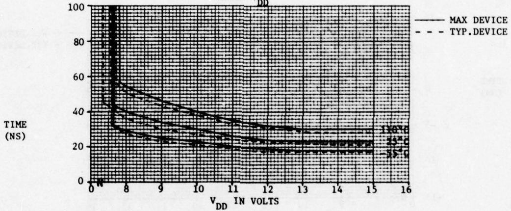
VERSUS TEMPERATURE
