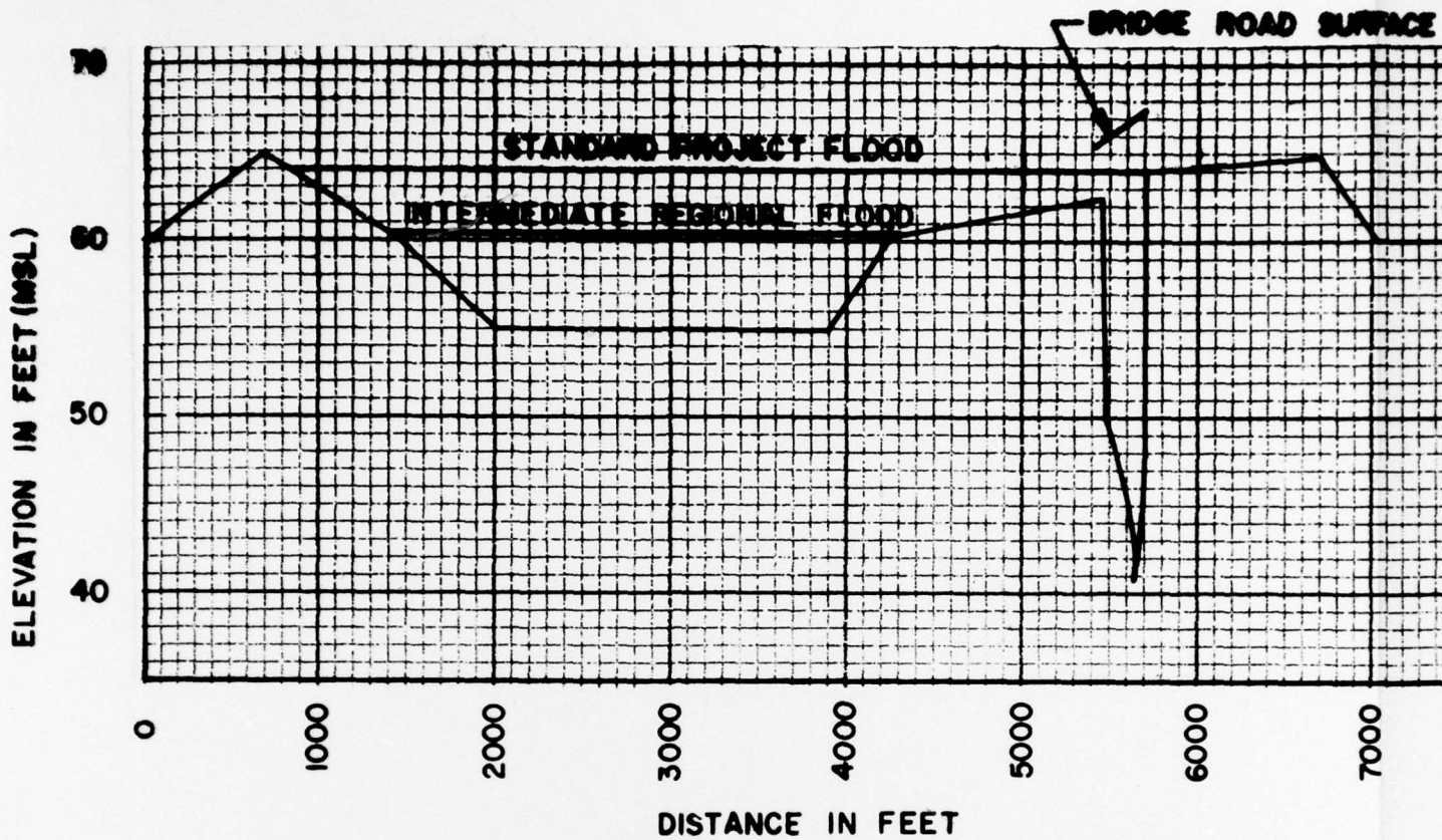
LOOP ROAD BRIDGE CROSS SECTIONS
