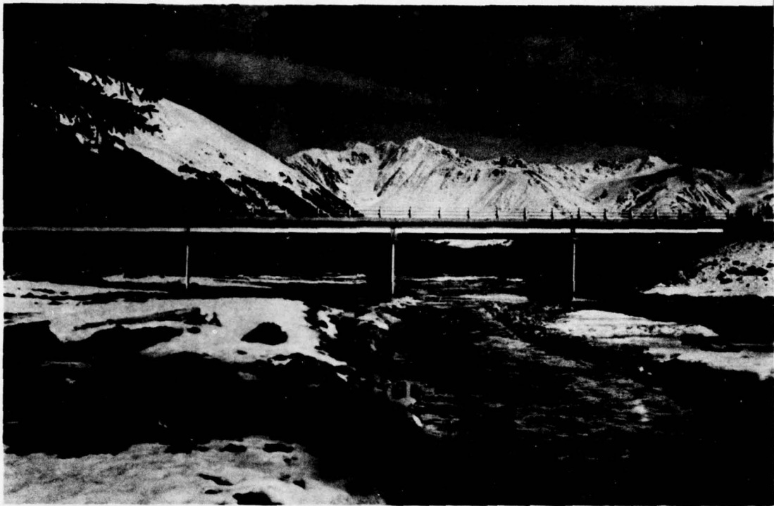
BRIDGE CROSSING GLACIER CREEK ON ALYESKA HIGHWAY WAS DESIGNED TO PASS THE INTERMEDIATE REGIONAL FLOOD
