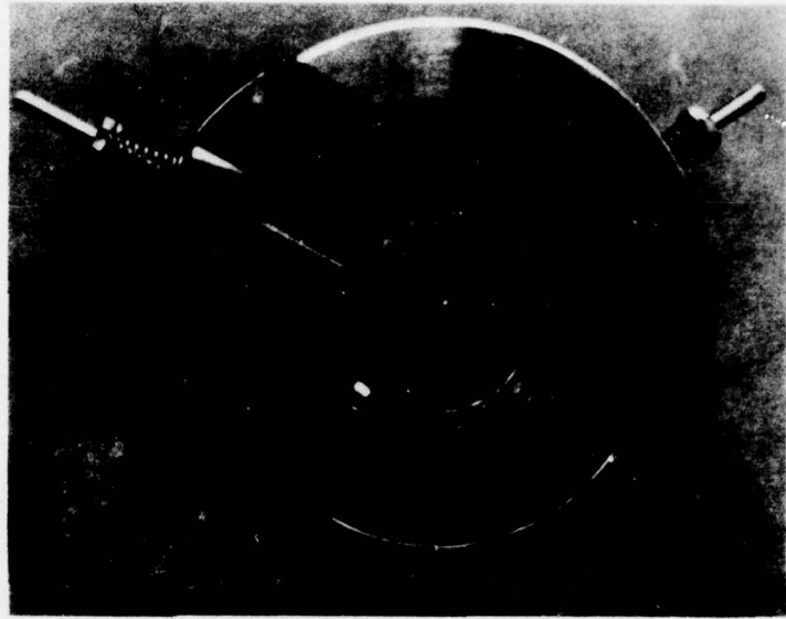
FIG. 4. Target-rod holding apparatus. The rod is supported by needle-pointed screws. The entire support system was spring-loaded to allow for thermal expansion.
