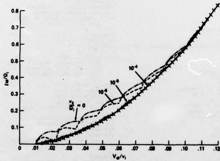
Fig. 2 - Plot of \gamma_m/\Omega_i vs. V_{di}/v_i for m_i = 16 m_p , T_e = T_i , \omega_{pe}/\Omega_e = 10.0 and \nu_{ii}/\Omega_i = 0.0 (---), 10^{-6} (---), 10^{-5} (.....) and 10^{-4} (x x x x). The solid line represents the lower-hybrid-drift instability.
