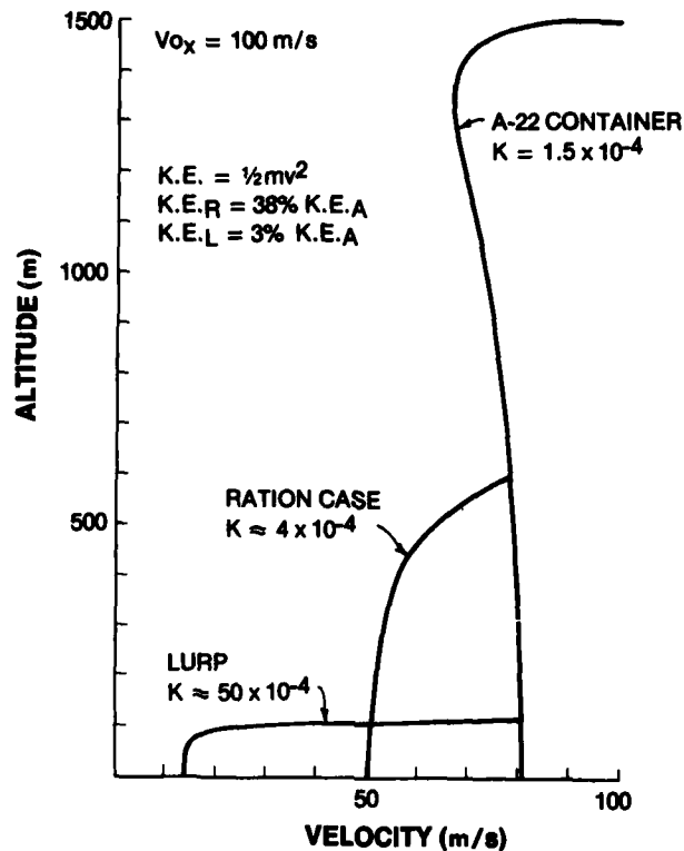
Figure 18. Effect of Mid-Air Dispersion on Impact Velocity
