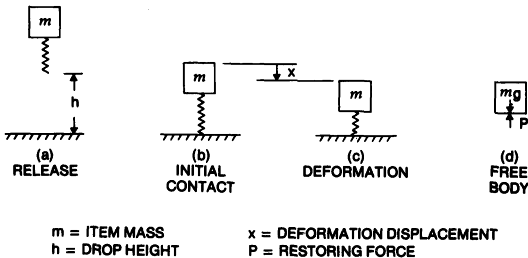
Figure 21. Elementary System
