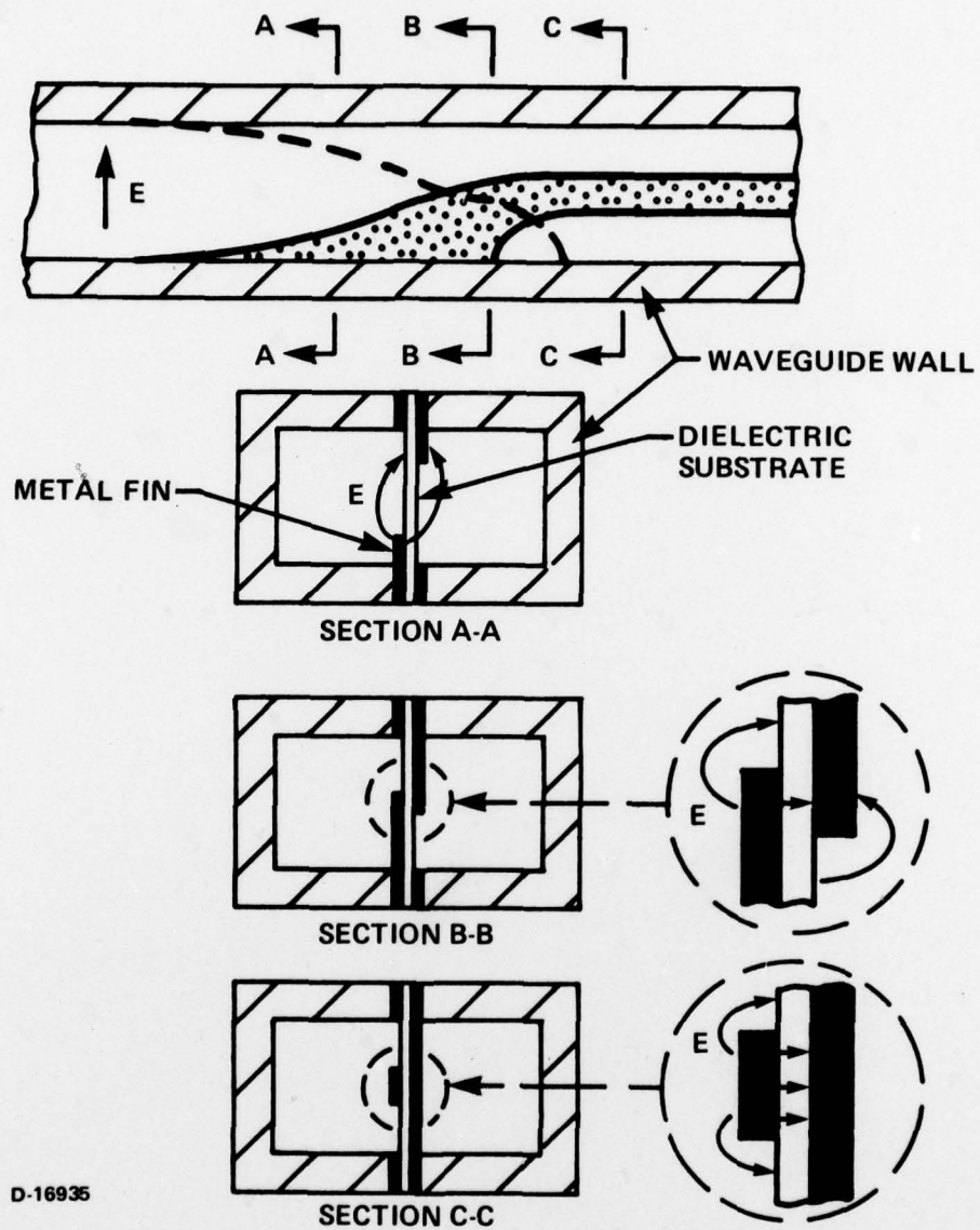
FIGURE 4.0.1 WAVEGUIDE-MICROSTRIP TRANSITION
