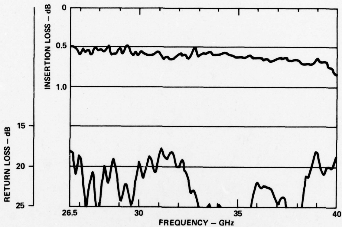
FIGURE 2.5.2 RESPONSE OF 50 \Omega LINE WITH DC BLOCKS IN FINAL SWITCH HOUSING
