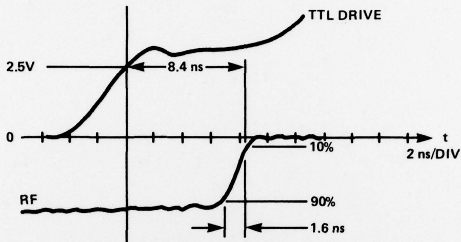
a) RF TURN-OFF TRANSIENT
