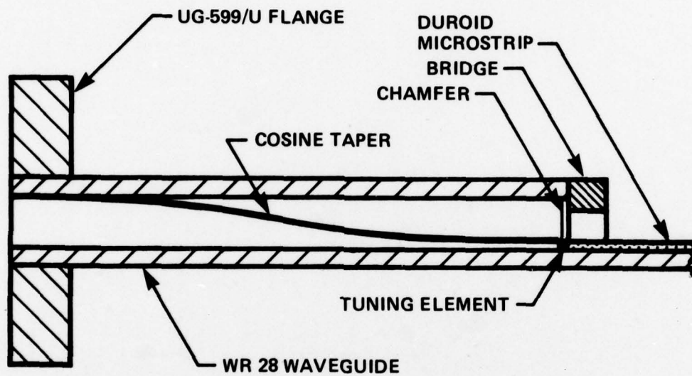
FIGURE 2.2.1 CROSS SECTION OF WAVEGUIDE-MICROSTRIP TAPERED TRANSITION
