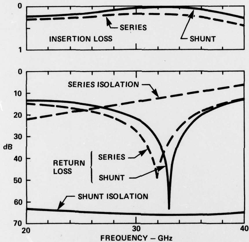
FIGURE 2.1.3 CHARACTERISTICS OF 2-DIODE SPST SWITCHES WITH .03 pF, 1\Omega DIODES IN SERIES AND SHUNT CONFIGURATIONS
