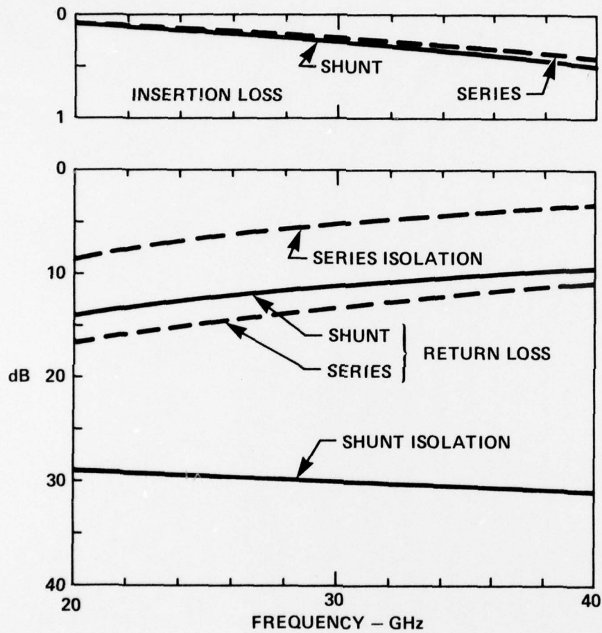
FIGURE 2.1.2 CHARACTERISTICS OF .03 pF, 1\Omega DIODE IN SERIES AND SHUNT MOUNTING
