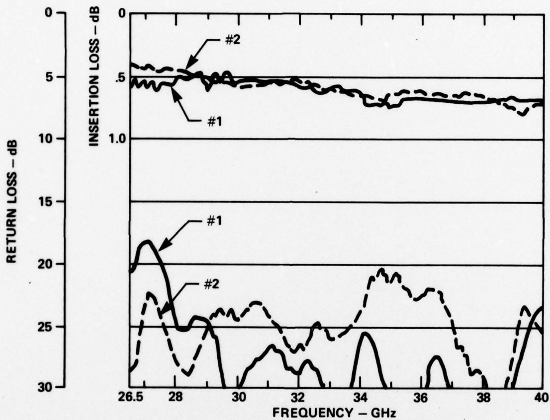
FIGURE 2.2.2 INSERTION & RETURN LOSS OF TWO MICROSTRIP TEST FIXTURES WITH 0.5" OF DUROID MICROSTRIP LINE
