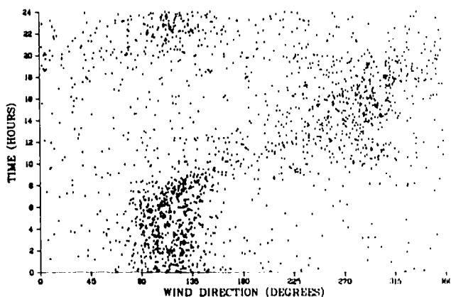
Fig. 10 - Wind direction at WAFB Station 2 versus time of day, June 1976 - June 1977
