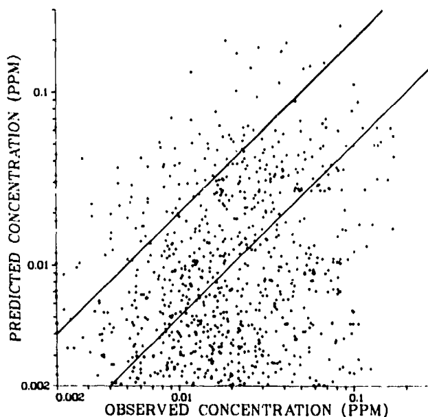
Fig. 15 - AQAM II predicted versus observed hourly average NO x concentrations, WAFB, January 1977 - parallel lines indicate factor of 2 level of agreement
