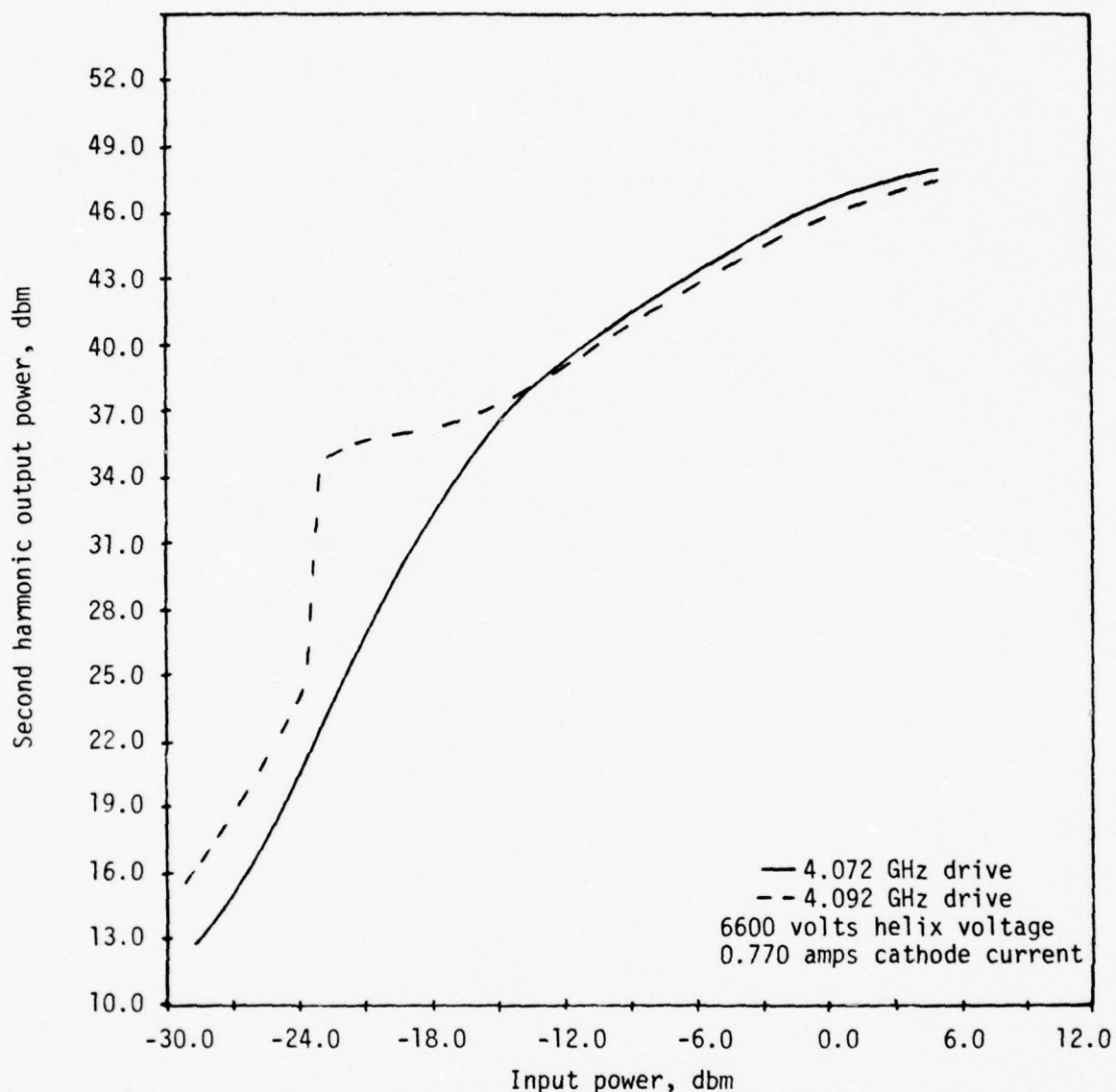
Figure 16c. Second harmonic output power vs. input power (driving at the fundamental) at two frequencies of interest. Solid line corresponds to input at 4.072 GHz, adjacent to but unaffected by the power hole. Dashed line corresponds to input at 4.092 GHz, the center of the power hole and drive-associated oscillation. At all points on both curves second harmonic output is at exactly twice the drive frequency.
