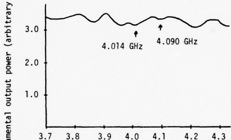
Figure 10h. Helix voltage =6400 volts.
