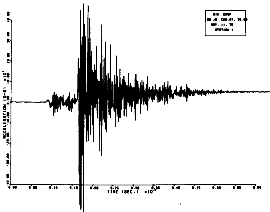
Figure 17. Fourier Spectrum and Corresponding Acceleration History, BP RIP Igniter
