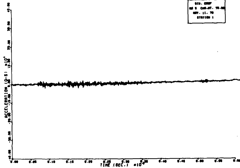
Figure 14. Fourier Spectrum and Corresponding Acceleration History, HIVE-LITE (90 kcal) Igniter
