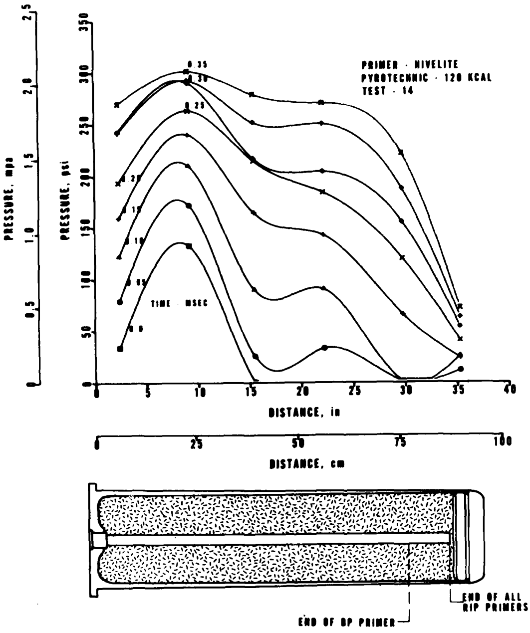
Figure 23. Pressure Distribution in an Inert Bed, HIVELITE (120 kcal) Igniter
