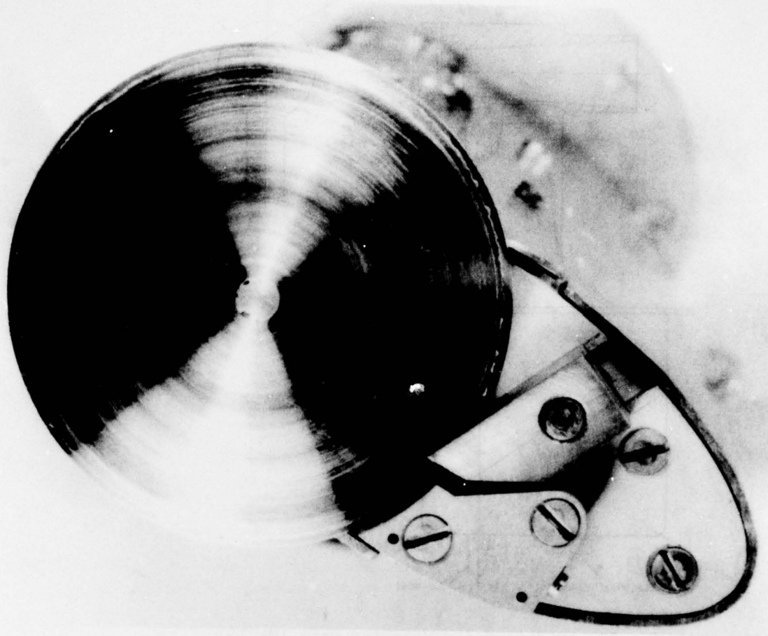
Fig 9 RAE rotating disc sensing head
