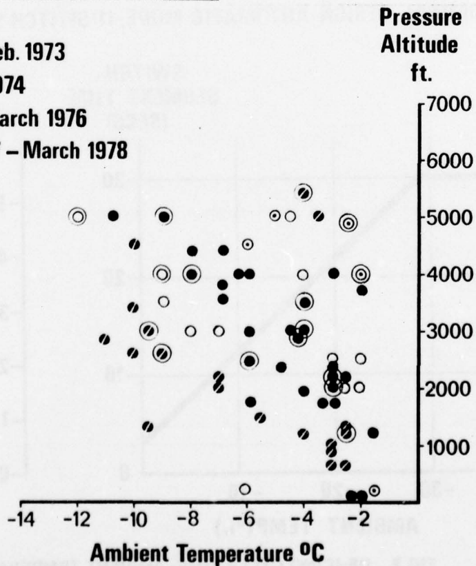
FIG.4. SUMMARY OF TESTS IN NATURAL ICING CONDITIONS
