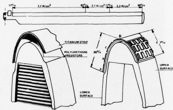
FIGURE 4 - SA.330 DE-ICED MAIN BLADE
