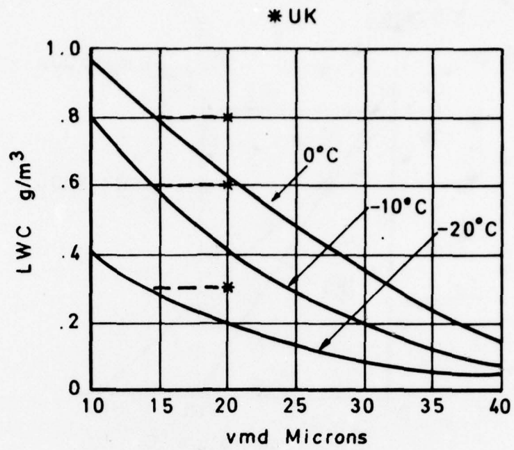
Fig 4 Continuous maximum
