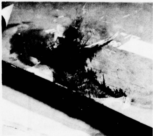
FIG. 10 : LIGHTNING STRIKE CURRENT TEST ON SA 330 MAIN BLADE
