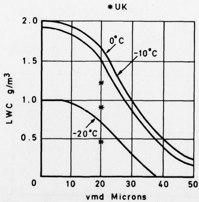
Fig 5 Intermittent maximum
