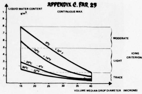
FIGURE 1 - F.A.R. 25 - CONTINUOUS MAX.
