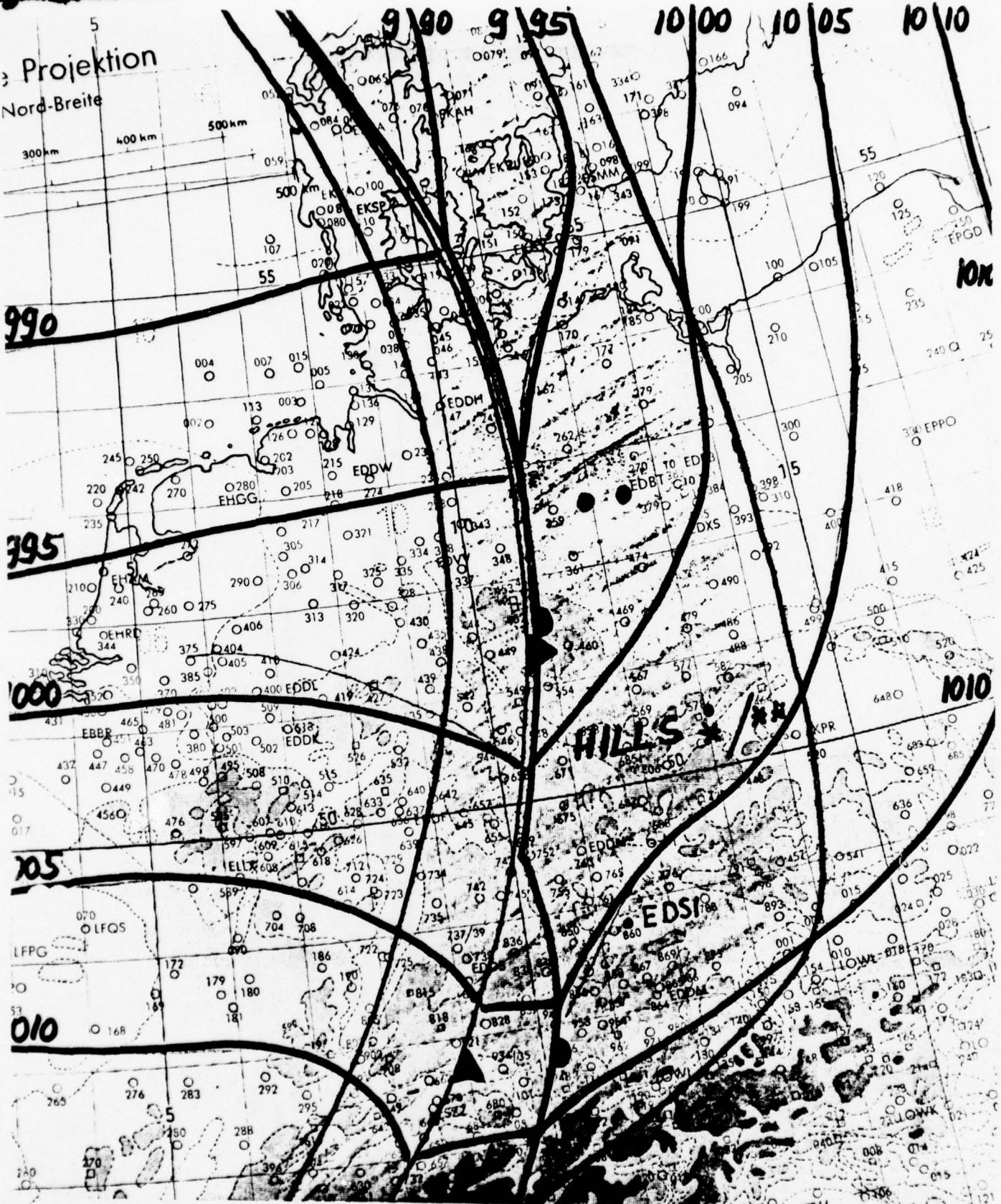
Figure 5: Meteorological situation
