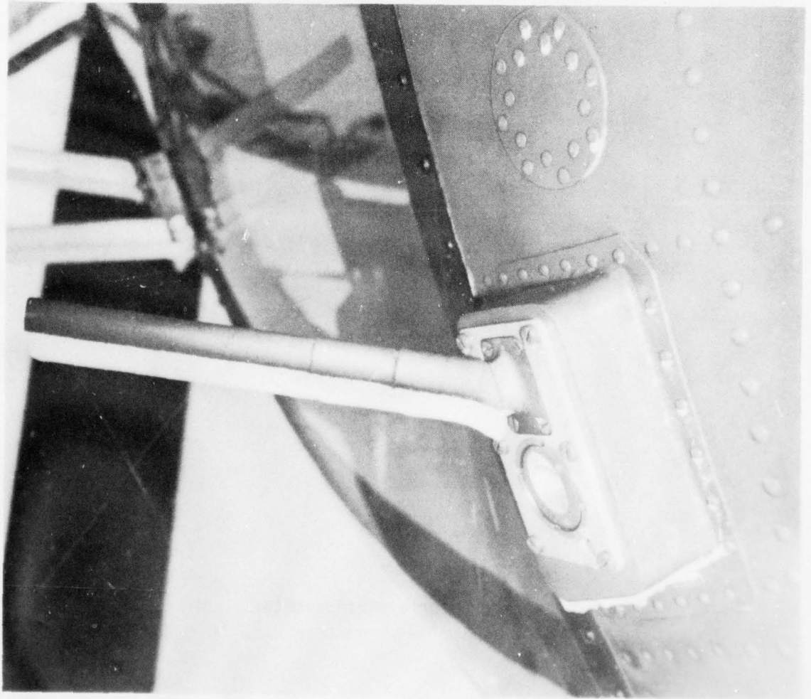
Fig 5 Accretion rod
