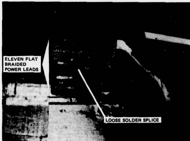
Figure 16. Station 80-83 Wiring Insulation Removed, Showing Spliced Wires and "Open" Joint That Were Found.
