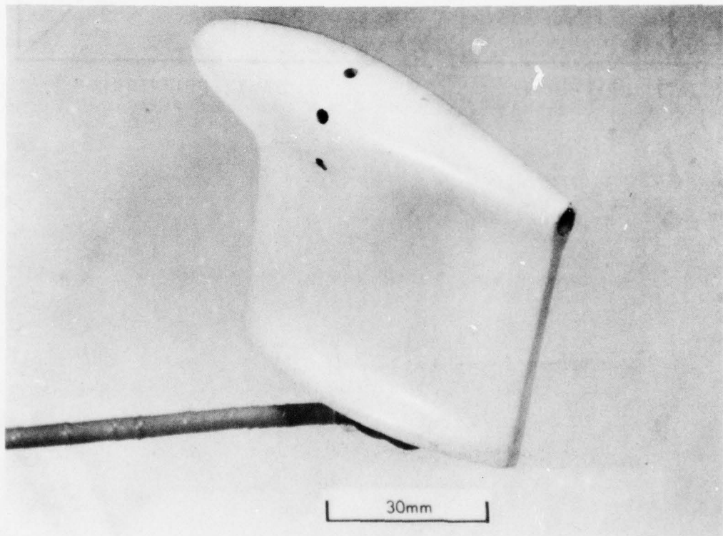
Fig 2 Rosemount oat sensing head
