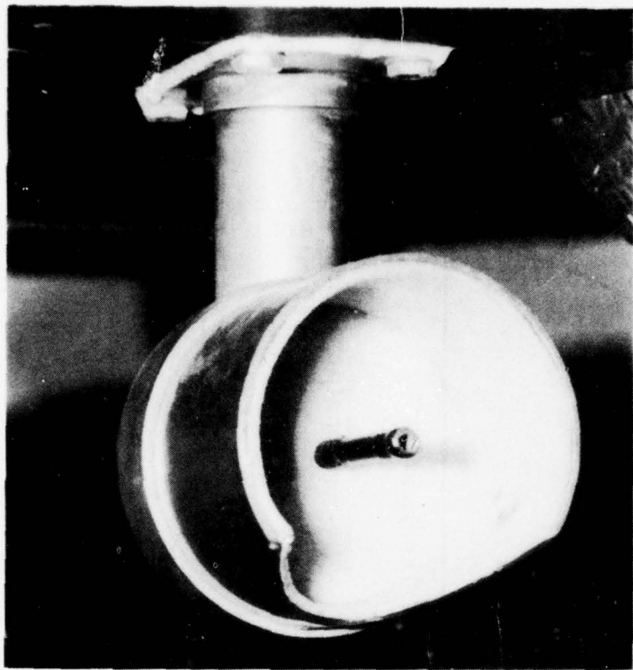
Fig 1 A&AEE oat sensing head
