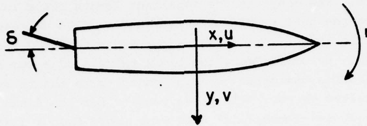
Figure 2. Definitions of coordinates, velocities, and rudder angle as viewed from the above.
