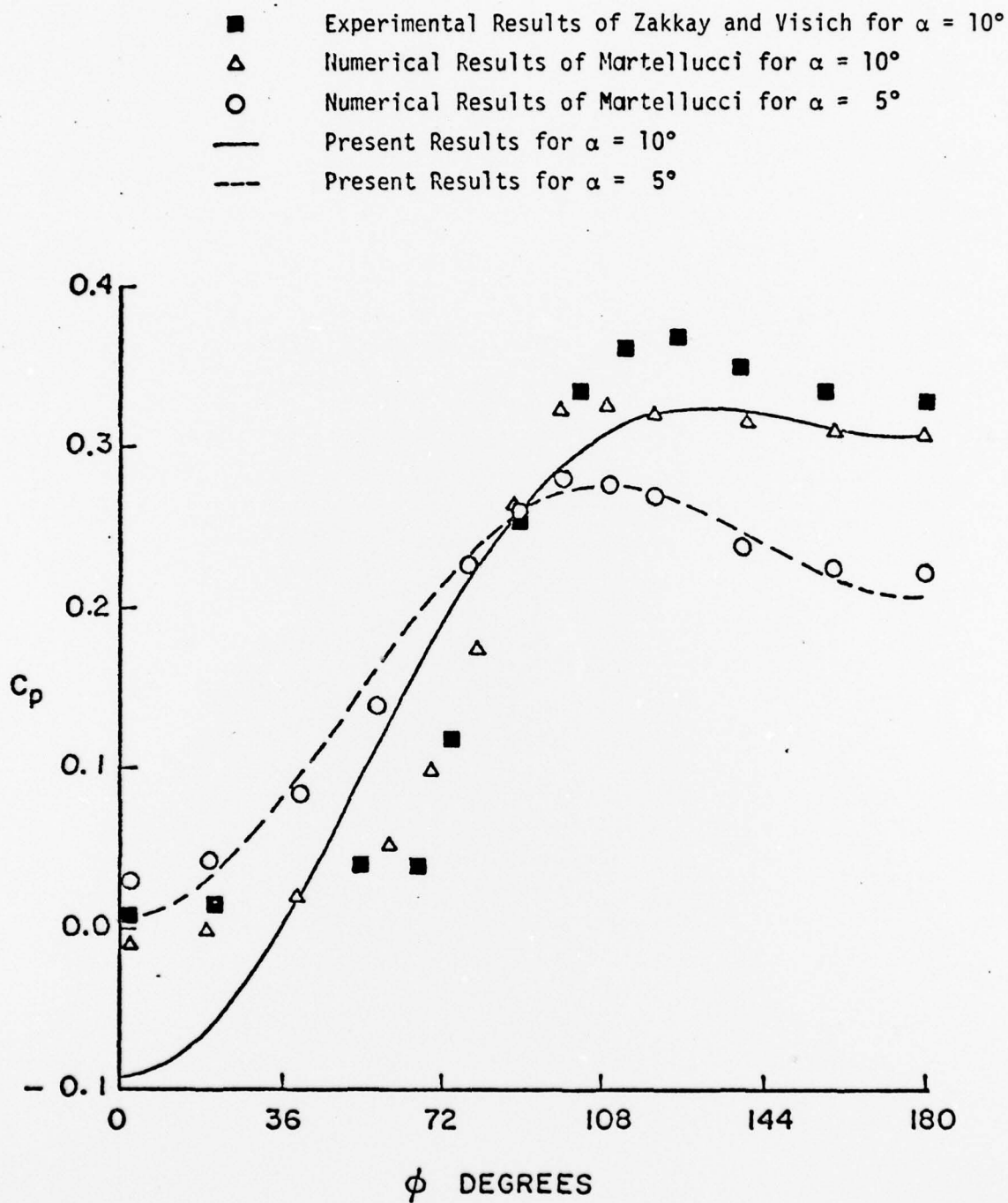
Figure 7.3. Comparison of Surface Pressure with Martellucci's Results, Model II, M_\infty = 6 , \gamma = 1.4
