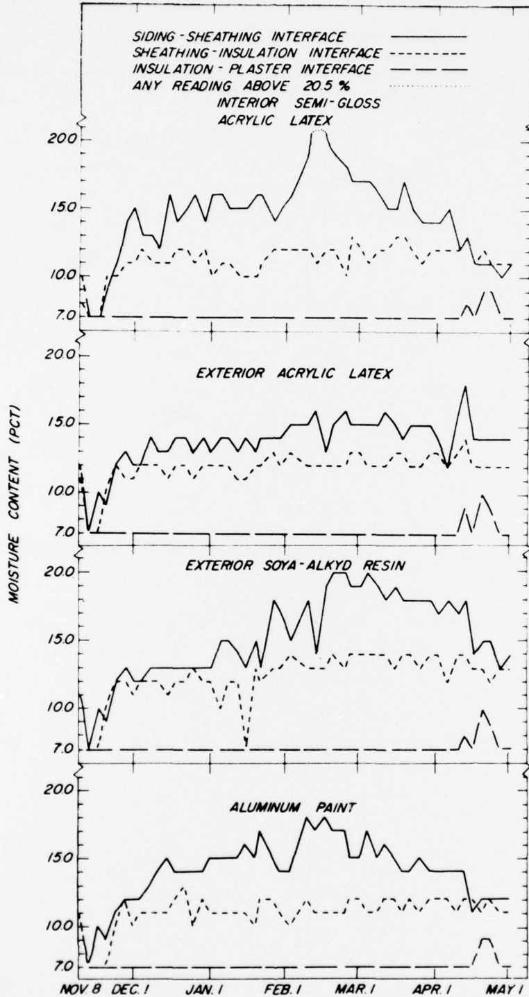
Figure 8. - - Moisture conditions through typical wall sections with paint applied to plaster for vapor resistance. (M 146 535)
