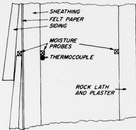
Figure 3. - - Cross section of stud space showing location of moisture probes and thermocouples. Probes were located at both one and seven feet from the floor. (M144 899)
