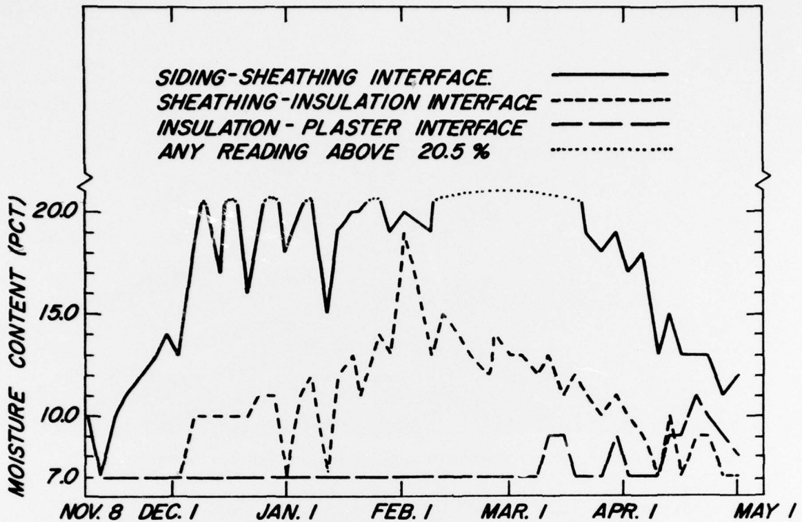
Figure 7. - - Moisture conditions through a typical wall section which incorporates no remedial measures. (M 146 537)
