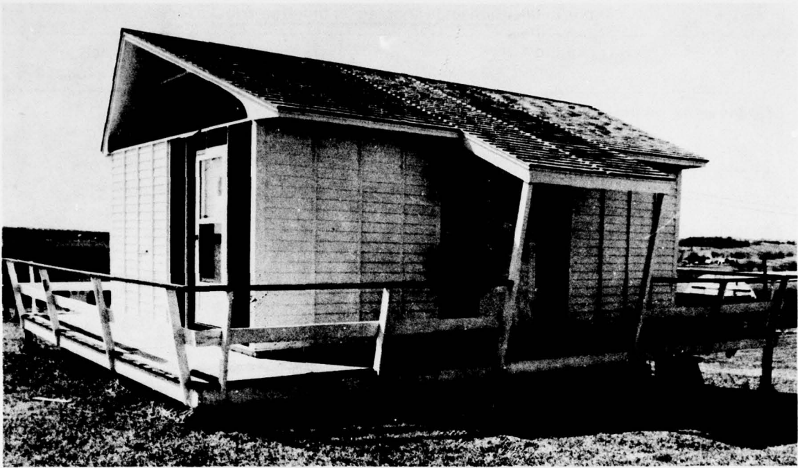
Figure 1. - - The U.S. Forest Products Laboratory test house located on the exposure site near Madison, Wis. (M 144 205-3)
