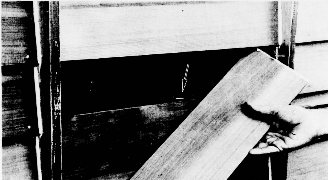
Figure 6. -- Moisture probe located immediately beneath siding. (M 142 642-9)
