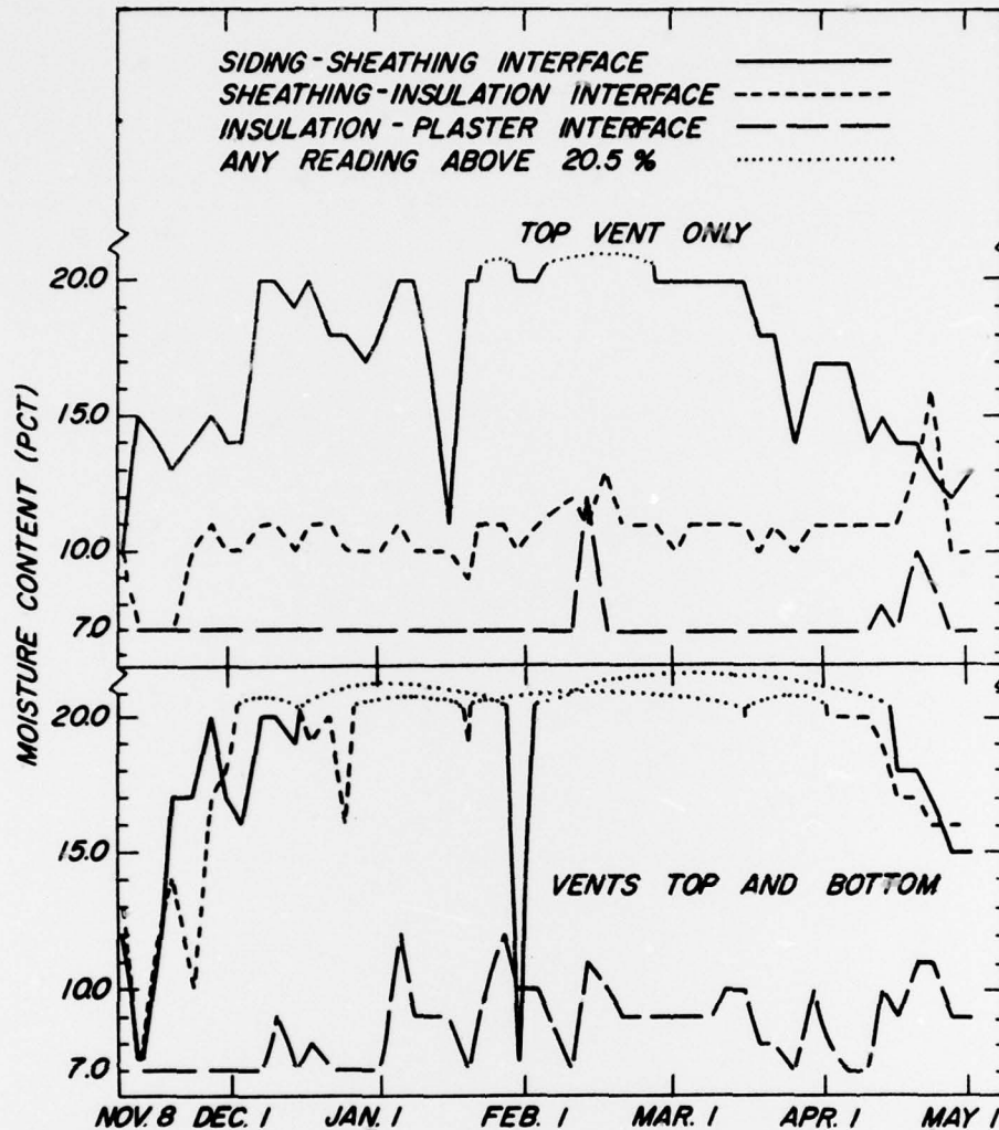
Figure 9. -- Moisture conditions through typical wall sections with 1-inch diameter vents in wall. (M 146 536)
