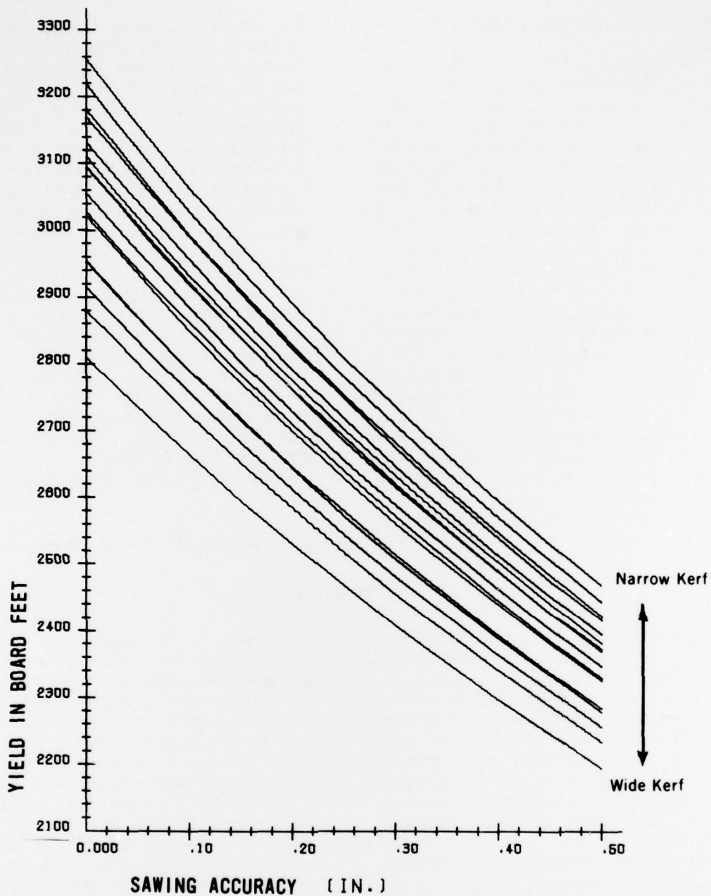
Figure 2.--Yield of a log sample showing effect of decreasing sawing accuracy in 16 combinations of vertical and horizontal kerf widths. The sample is composed of one log of each 1-inch diameter class.
