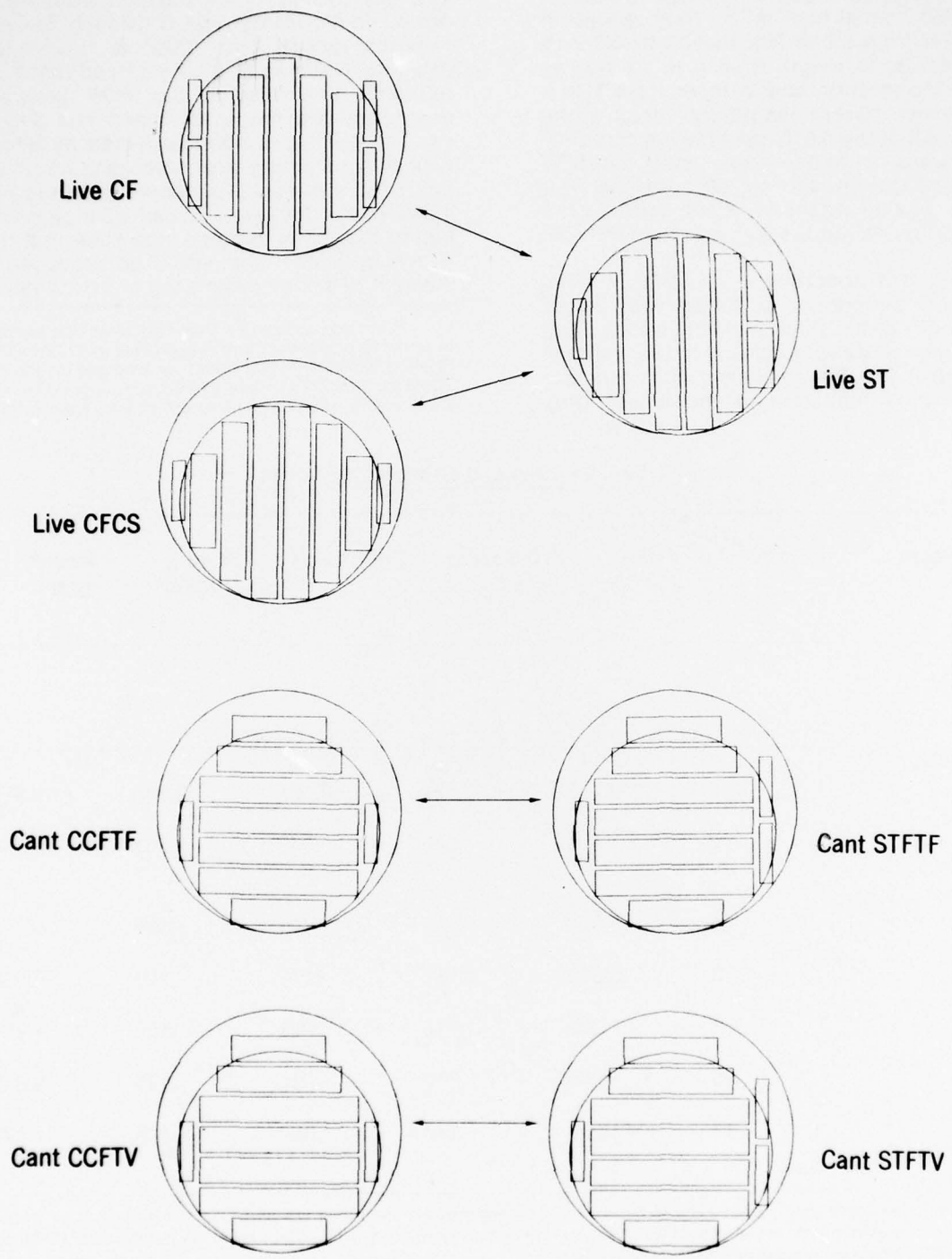
Figure 1.--The four centered sawing methods and the three counterpart offset methods with which they are compared.
