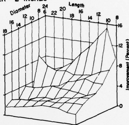
TAPER = 2 INCHES
