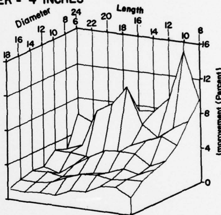
TAPER = 4 INCHES
