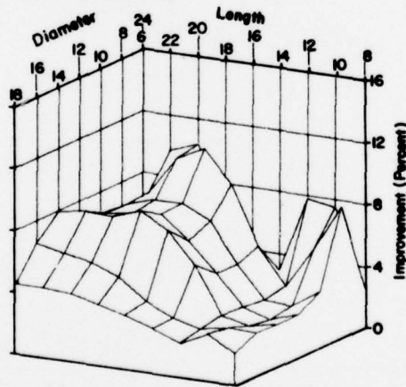
Figure 8.--The interaction between length, diameter, and the difference in yield between cant STFTF and cant CCFTF sawing methods by taper classes. (M 146 507)
