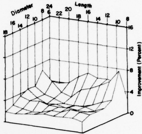
TAPER = 2 INCHES
