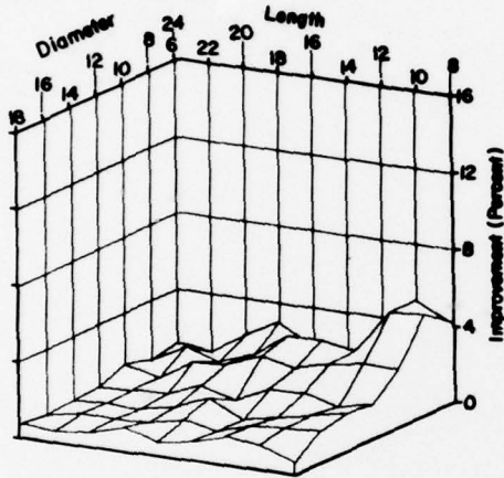
TAPER = 3 INCHES
