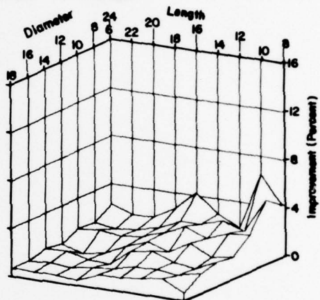
TAPER = 4 INCHES
