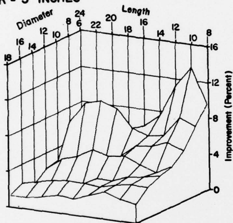
TAPER = 5 INCHES
