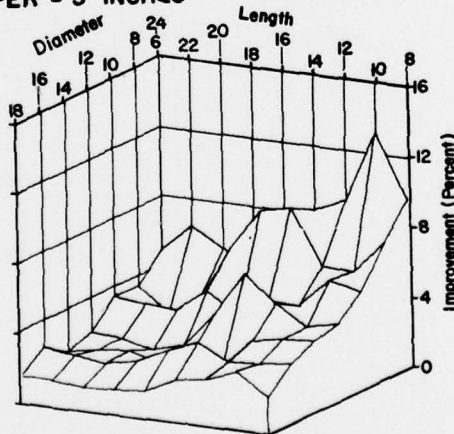
Figure 6--The interaction between length, diameter, and the difference in yield between live ST and live CF sawing methods by taper classes. (M 146 505)
