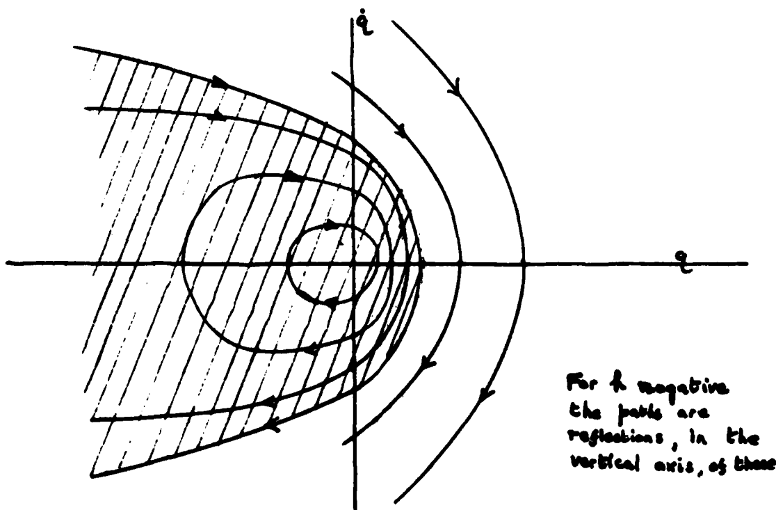
Fig 2. \ddot{q} + b\dot{q}^2 + cq = 0 \quad b, c > 0
