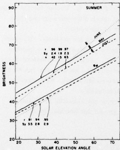
Figure 5. Graph of the Regression Equation for Average ( \bar{B} ) and Minimum ( B_m ) Ground Brightness vs. Solar Elevation Angle on Clear Days for Stations Indicated on Graph for May, June and July 1977. Note that r is the correlation coefficient; S_y , the standard error of estimate; and n , the number of cases
