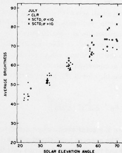
Figure 2. Scatter Diagram of Average Ground Brightness of 9 \times 9 Pixel Boxes Centered at the Four Test Stations During Clear and Scattered Conditions. (See text for definition of brightness)
