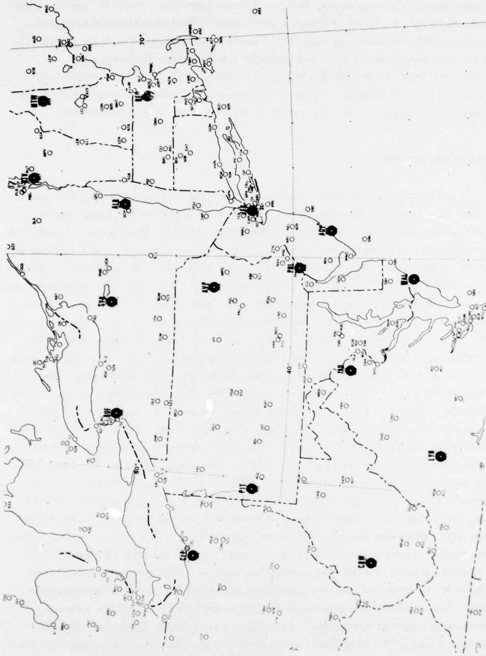
Figure 1. Area of Satellite Imagery Data. Surface reports saved for stations with bold markings
