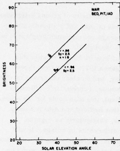
Figure 3. Graph of the Regression Equation for Average ( \bar{B} ) and Minimum ( B_m ) Ground Brightness vs. Solar Elevation Angle on Clear Days for Stations Indicated on Graph for March 1977. Note that r is the correlation coefficient; S_y , the standard error of estimate; and n , the number of cases
