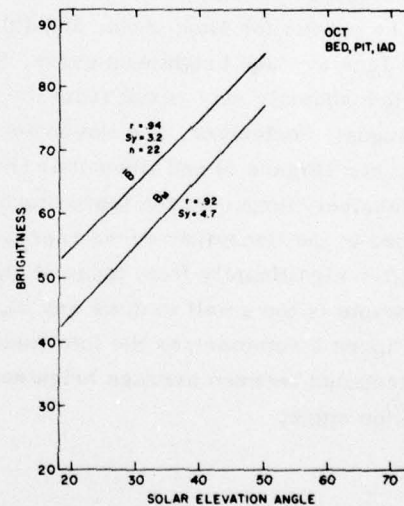
Figure 6. Graph of the Regression Equation for Average ( \bar{B} ) and Minimum ( B_m ) Ground Brightness vs. Solar Elevation Angle on Clear Days for Stations Indicated on Graph for October 1977. Note that r is the correlation coefficient; S_y , the standard error of estimate; and n , the number of cases.
