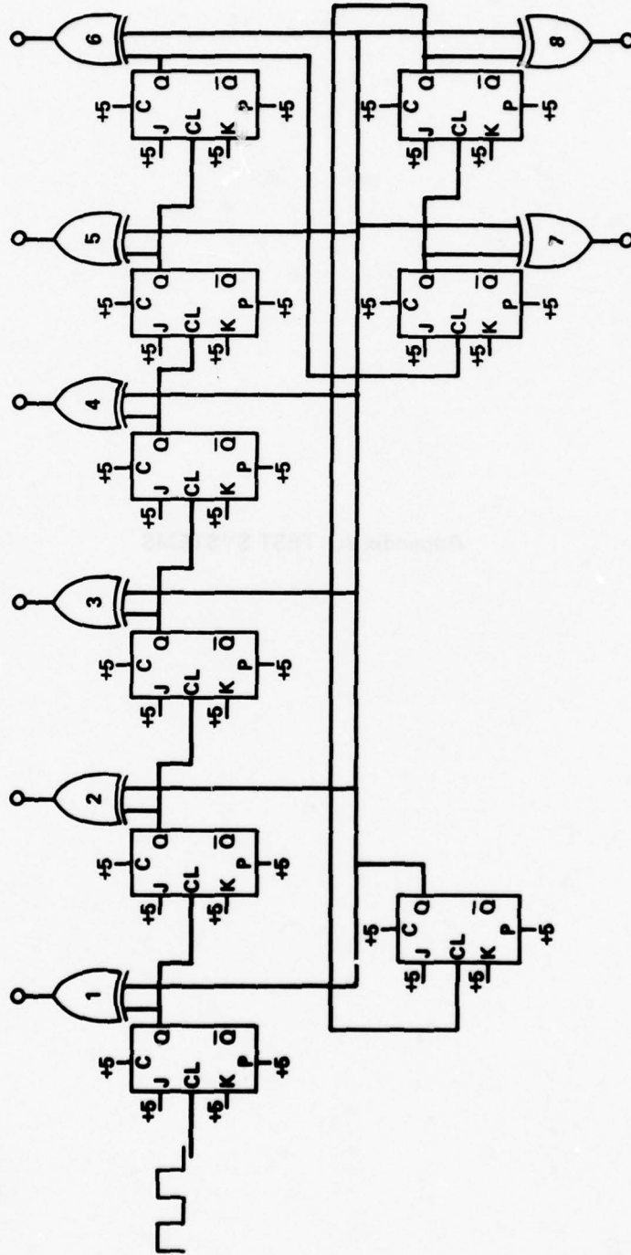
UP AND DOWN COUNTER (8 bytes)
