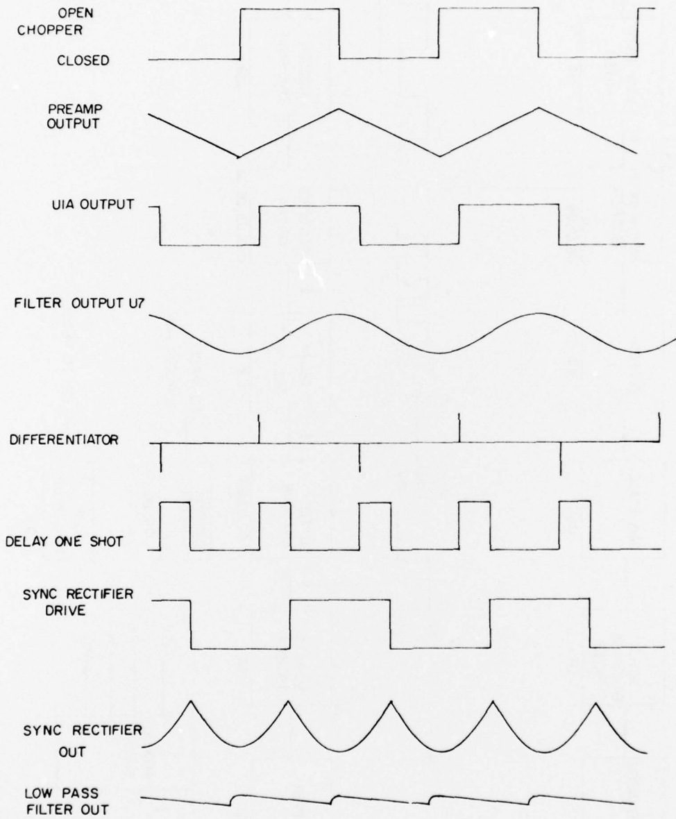
Figure 2-2. Timing Diagram.
