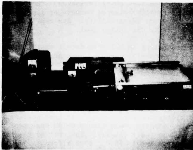
B. Scanner Board and Parallel X-Y Plotter.
