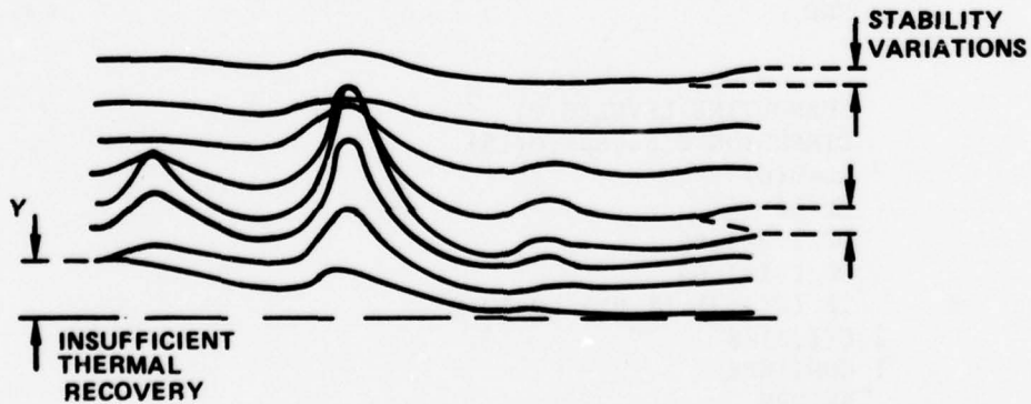
Figure 7. Analog trace of the LEECO Corporation's LCP200T sensor showing instability and poor thermal recovery.
