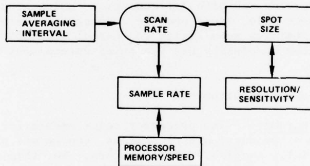
Figure 3. Parameters which affect scan rate.
