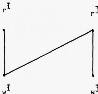
A Conflict Graph Illustrating P1
