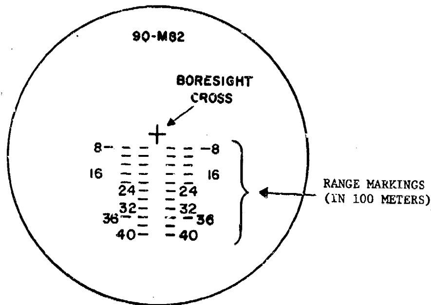
Figure 1. Ballistic Reticle.
