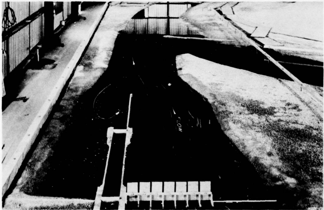
Photo 9. Plan E; discharge 58,000 cfs, lower pool el 56.2. Surface current direction; note eddy in lower lock approach
