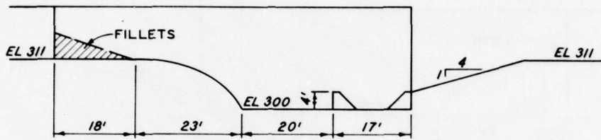
ELEVATION TYPE 7
