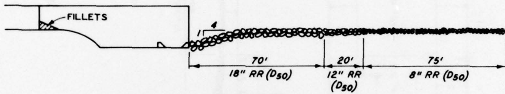
ELEVATION TYPE 14C
