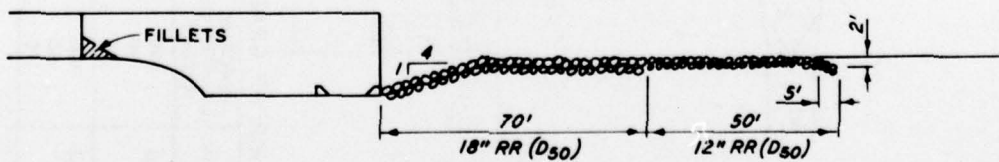
ELEVATION TYPE 14D
