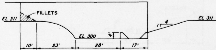
ELEVATION TYPE 9
