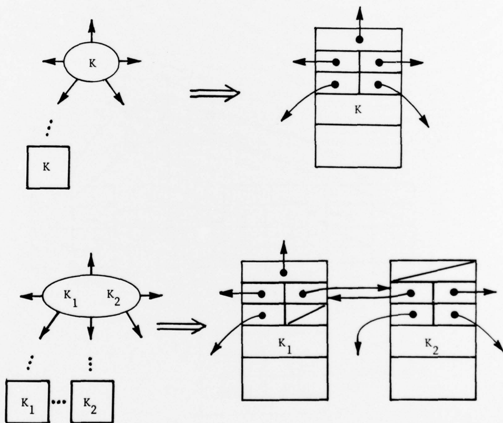
Figure 9. A storage representation for internal and external nodes.
