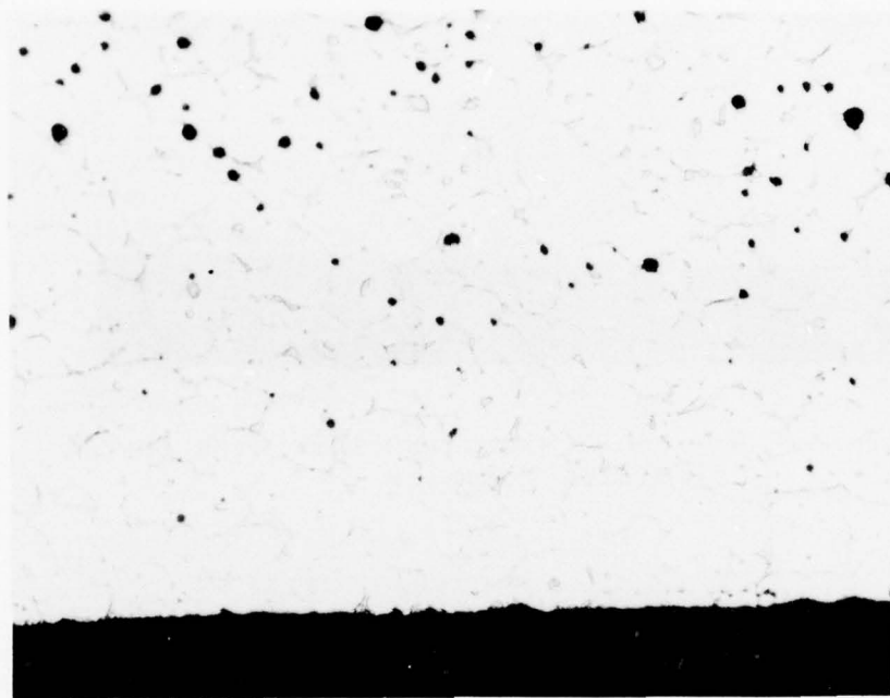
Figure 5. Brazed S1 Microstructure After Diffusion Treatment
