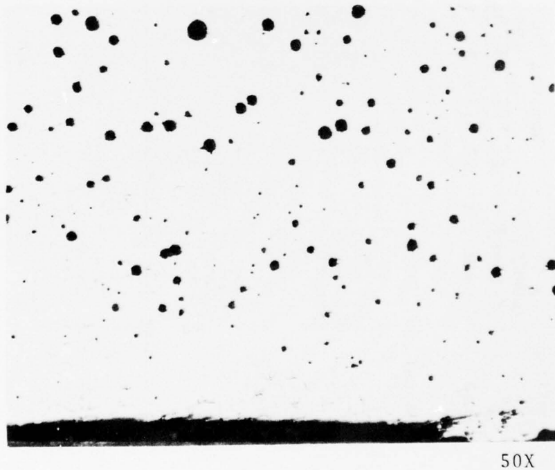
Figure 2. Brazed Si Microstructure with Highest Calculated Porosity
