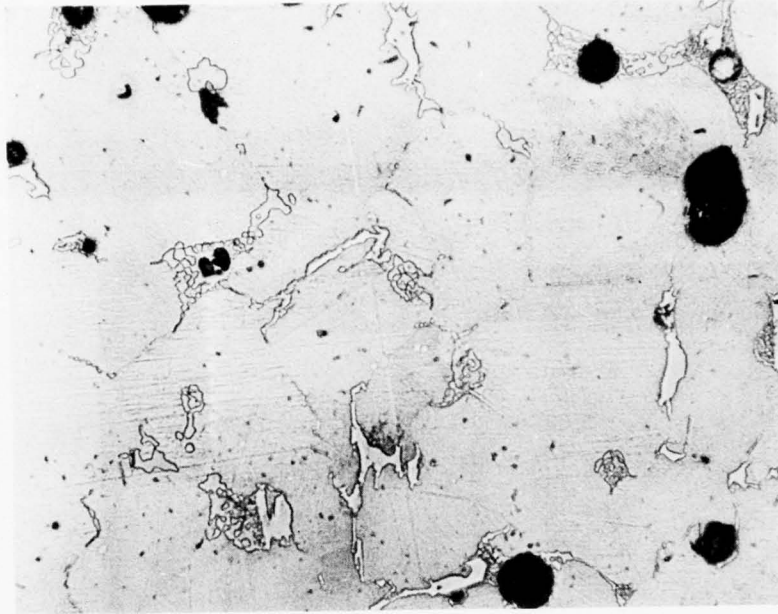
b. Kallings Etch 200X
