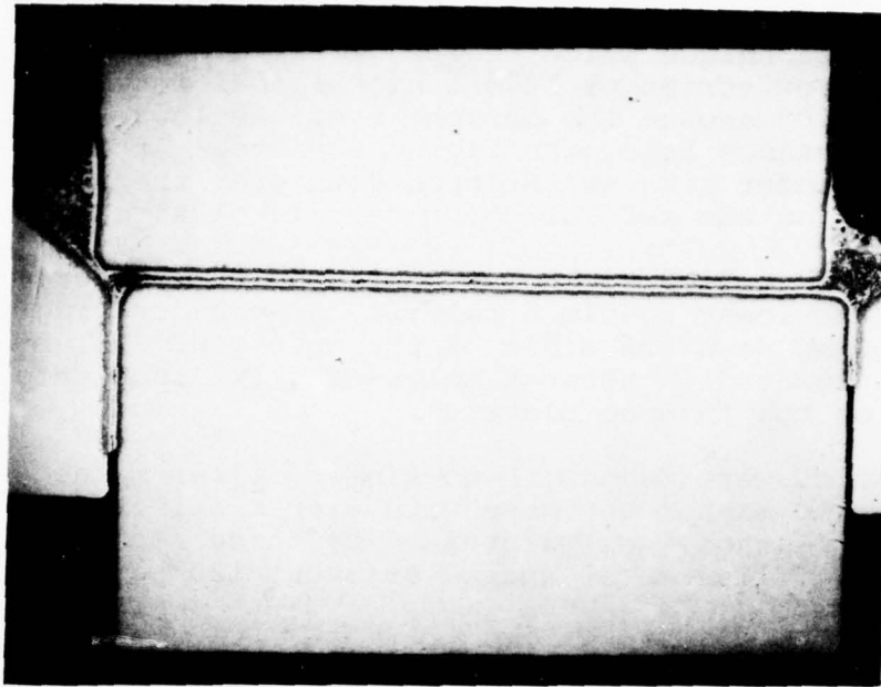
Figure 15. Typical Braze Joint with No Sinter Filler Metal for Small Joint Clearance, 9 mil
