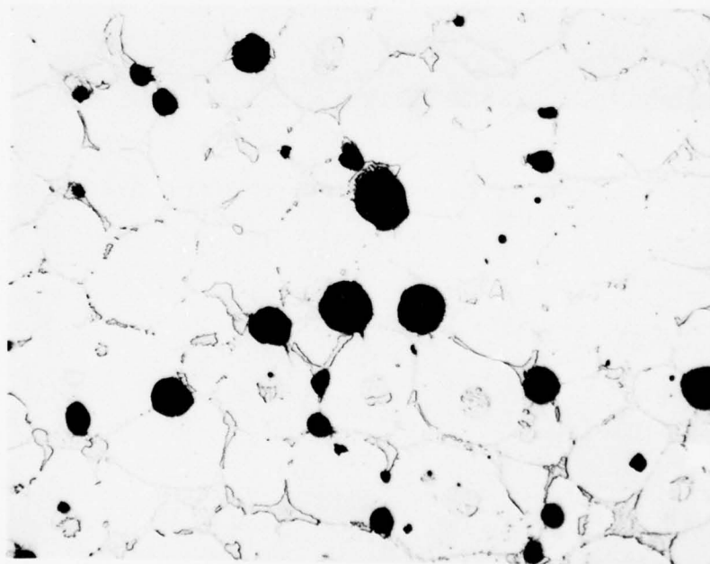
Figure 4. Brazed Specimen Showing Relationship of Porosity and Interstitial Phase
